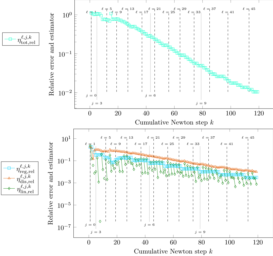
Figure 10: [Unknown singular solution with data (10.4), kink nonlinearity (2.19) with s_0 = 0.75 and m = 10000 , final #DOFs = 86973, \epsilon^0 = 0.125 , \gamma_{\text{reg}} = 0.4 , \gamma_{\text{lin}} = 0.4 , C_\epsilon = 0.5 , polynomial degree p = 1 , mesh refinement index \ell , regularization index j , linearization index k ] Applying Algorithm 1 using adaptive refinement.
