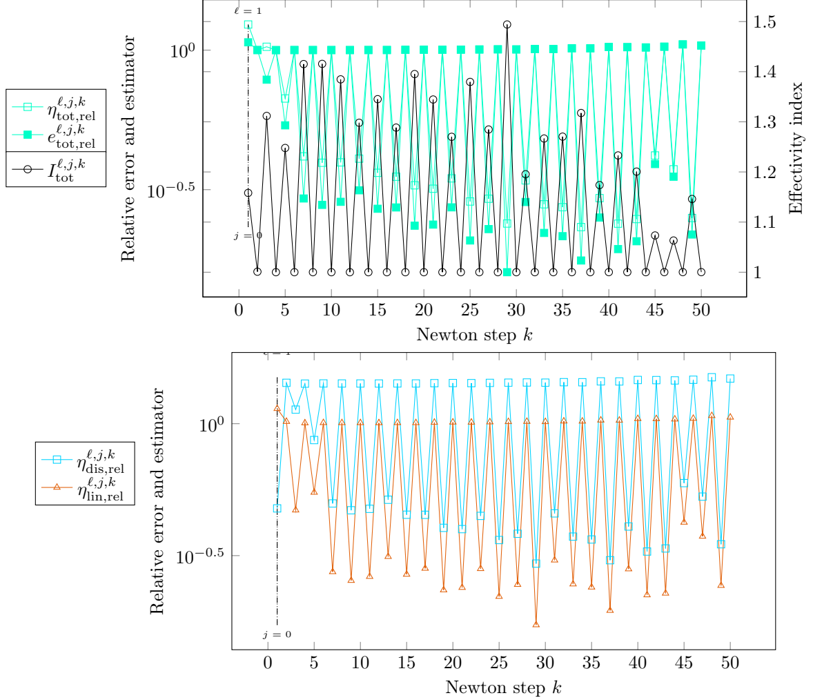
Figure 5: [Polynomial solution (10.3), kink nonlinearity (2.19) with s_0 = 1 and m = 10000 , polynomial degree p = 1 , #DOFs = 261121, no regularization \epsilon^0 = 0 , refinement index \ell , regularization index j , linearization index k , ] The classical Newton method fails to converge for the unregularized problem corresponding to \epsilon = 0 .
