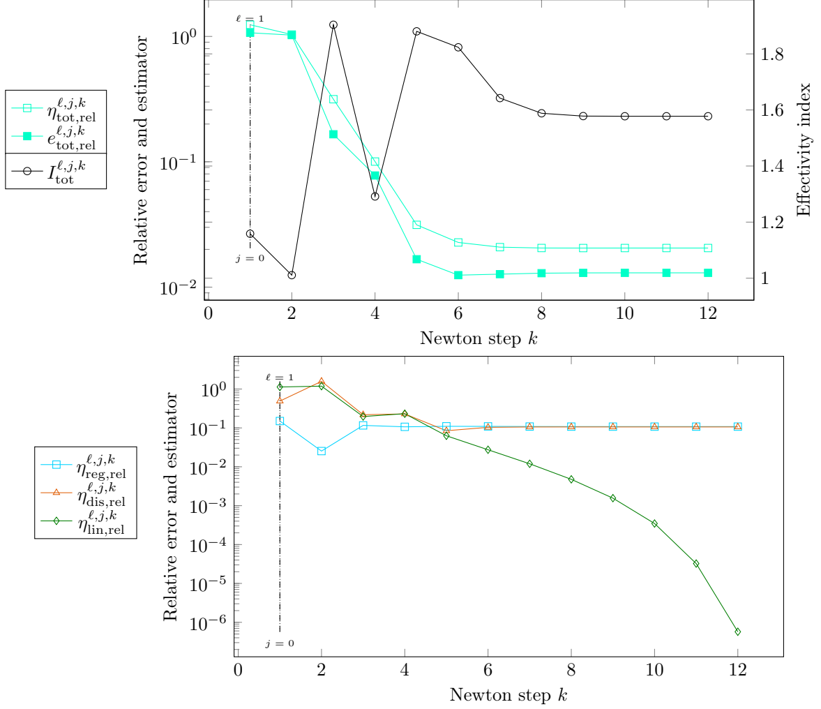
Figure 6: [Polynomial solution (10.3), kink nonlinearity (2.19) with s_0 = 1 and m = 10000 , #DOFs = 261121, \epsilon^0 = 0.125 , \gamma_{\text{reg}} = 1.0\text{e}16 , \gamma_{\text{lin}} = 1.0\text{e}5 , C_\epsilon = 1 , polynomial degree p = 1 , mesh refinement index \ell , regularization index j , linearization index k ] The classical Newton method converges for the regularized problem with \epsilon = 0.125 but the level of regularization possibly pollutes the error due the discretization.
