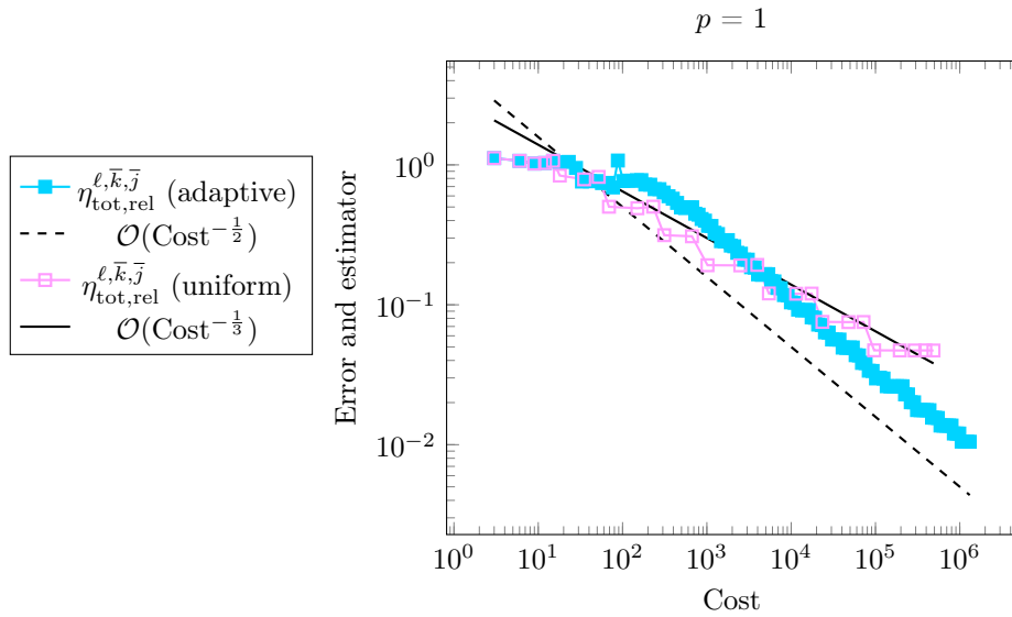
Figure 14: [Unknown singular solution with data (10.4), kink nonlinearity (2.19) with s_0 = 0.75 and m = 10000 , polynomial degree p = 1 , \epsilon^0 = 0.125 , \gamma_{\text{reg}} = 0.4 , \gamma_{\text{lin}} = 0.4 , C_\epsilon = 0.5 , #DOFs varies] Convergence in costs given by the triple sum (10.5). We observe the same rates in function of the cost as we do for the DOFs which is expected theoretically.
