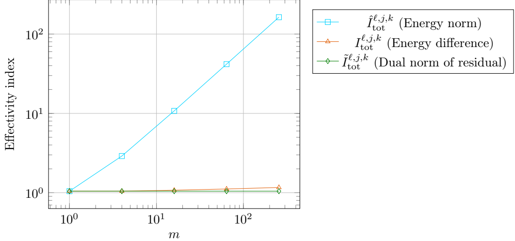
Figure 4: [Polynomial solution (10.3), kink nonlinearity with s_0 = 1 and m varying, polynomial degree p = 1 , #DOFs=3969, no regularization \epsilon = 0 ] The effectivity associated with the energy norm scales linearly in m whereas the other effectivities remain constant.
