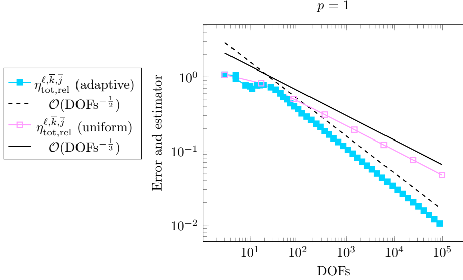
Figure 11: [Unknown singular solution with data (10.4), kink nonlinearity (2.19) with s_0 = 0.75 and m = 10000 , polynomial degree p = 1 , \epsilon^0 = 0.125 , \gamma_{\text{reg}} = 0.4 , \gamma_{\text{lin}} = 0.4 , C_\epsilon = 0.5 , #DOFs varies] Comparison of the suboptimal convergence for uniform refinement and optimal convergence for adaptive mesh refinement based on the estimator \eta_{\text{tot}}^{\ell,j,k} for the lowest order.
