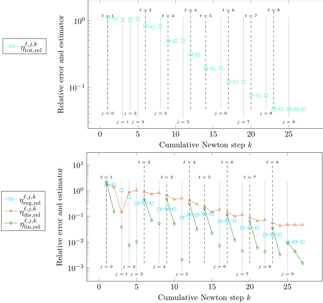
Figure 9: [Unknown singular solution with data (10.4), kink nonlinearity (2.19) with s_0 = 0.75 and m = 10000 , final #DOFs = 97793, \epsilon^0 = 0.125 , \gamma_{\text{reg}} = 0.4 , \gamma_{\text{lin}} = 0.4 , C_\epsilon = 0.5 , polynomial degree p = 1 , mesh refinement index \ell , regularization index j , linearization index k ] Applying Algorithm 1 using uniform refinement.
