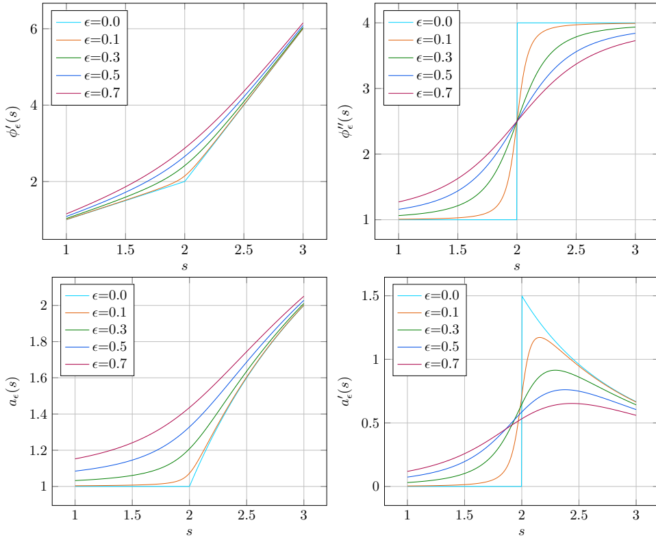
Figure 2: [Kink function (2.19) with m = 4 , s_0 = 2 ] Regularization of the kink function (2.19) by replacing the absolute value function with its differentiable counterpart, see (2.25).
