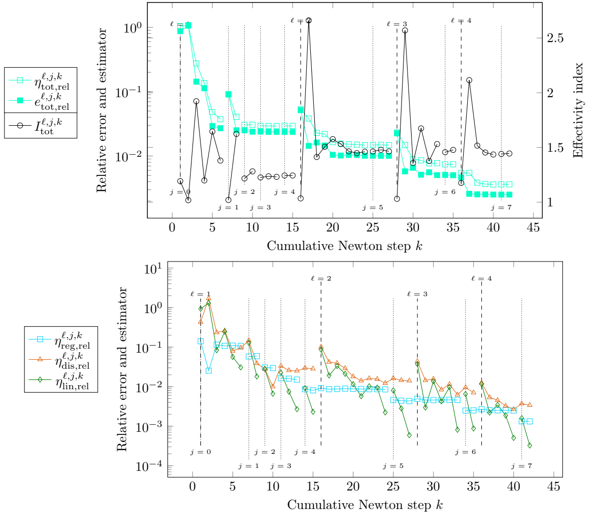
Figure 7: [Polynomial solution (10.3), kink nonlinearity (2.19) with s_0 = 1 and m = 10000 , final #DOFs = 261121, \epsilon^0 = 0.125 , \gamma_{\text{reg}} = 0.6 , \gamma_{\text{lin}} = 0.4 , C_\epsilon = 0.5 , polynomial degree p = 1 , mesh refinement index \ell , regularization index j , linearization index k ] The adaptive Algorithm 1 applied to a polynomial solution. The final value of the regularization parameter is \epsilon^6 = 1.95\text{e-}3 .
