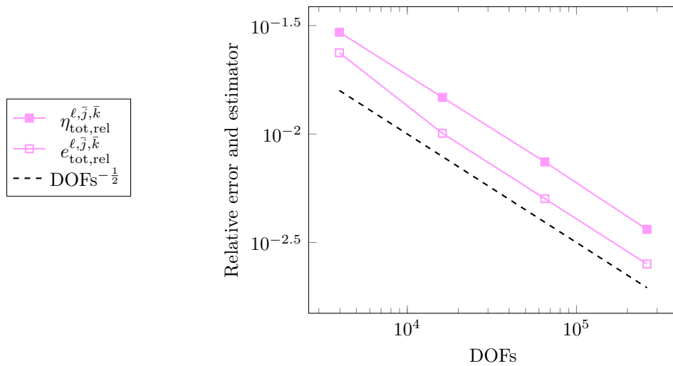
Figure 8: [Polynomial solution (10.3), kink nonlinearity (2.19) with s_0 = 1 and m = 10000 , polynomial degree p = 1 , \epsilon^0 = 0.125 , \gamma_{\text{reg}} = 0.6 , \gamma_{\text{lin}} = 0.4 , C_\epsilon = 0.5 , #DOFs varies] Achieving the optimal rate of convergence for a polynomial solution with uniform mesh refinement.
