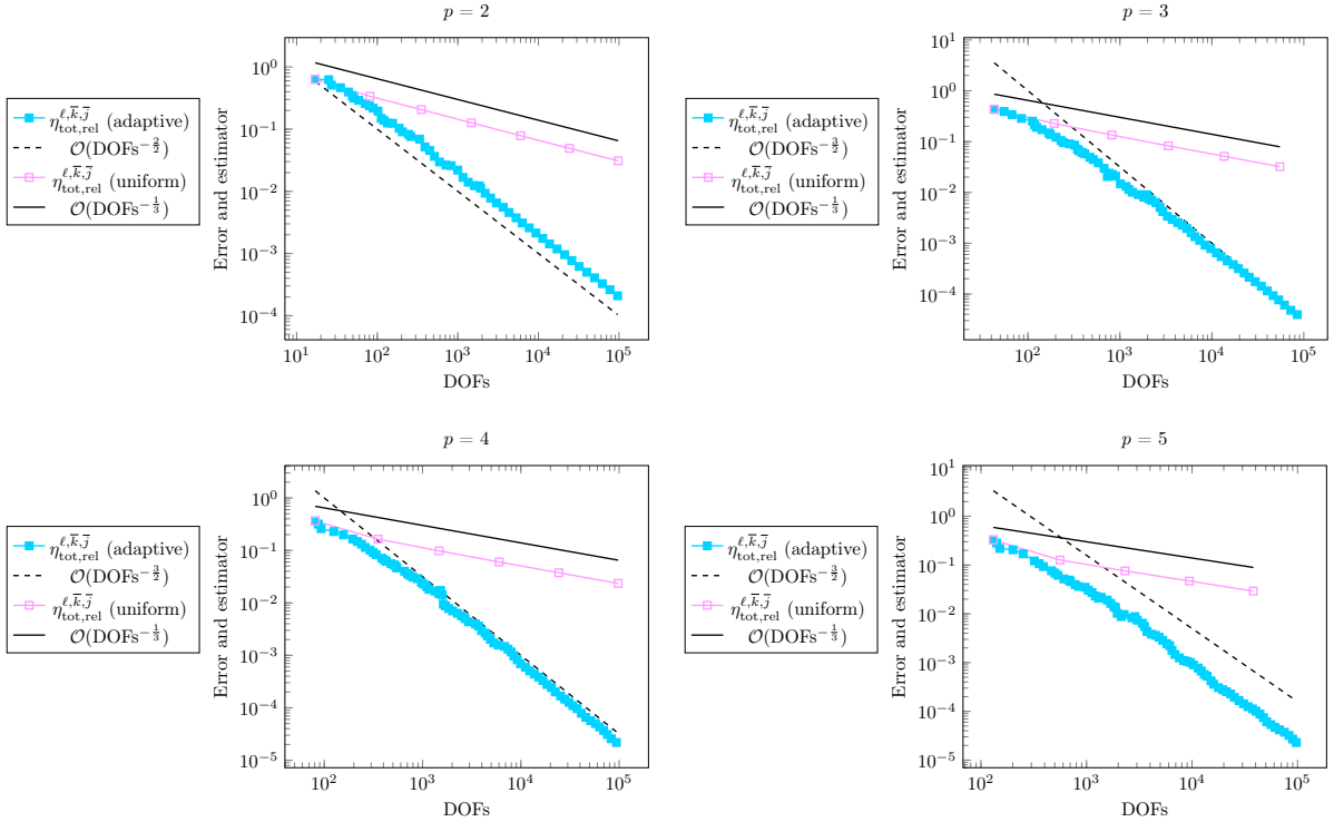
Figure 12: [Unknown singular solution with data (10.4), kink nonlinearity (2.19) with s_0 = 0.75 and m = 1000 , different polynomial degrees p , #DOFs varying, \epsilon^0 = 0.125 , \gamma_{\text{reg}} = 0.4 , \gamma_{\text{lin}} = 0.4 , C_\epsilon = 0.5 ] Different polynomial degrees p using adaptive mesh refinement based on \eta_{\text{tot}}^{\ell,j,k} . The optimal rate of \text{DOFs}^{-p/d} is obtained for adaptive refinement up to p = 3 , then only suboptimal convergence of \text{DOFs}^{-3/d} is achieved. We explain this by the appearance of one-dimensional (curve) singularities. In the case of uniform mesh refinement, increasing the polynomial degree does not change the suboptimal rate of \text{DOFs}^{-1/3} .
