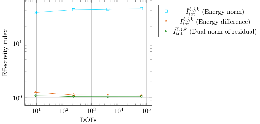
Figure 3: [Polynomial solution (10.3), kink nonlinearity (2.19) with s_0 = 1 and m = 64 , polynomial degree p = 1 , #DOFs varying, no regularization \epsilon = 0 ] Robustness with respect to the number of DOFs for the three error measures.
