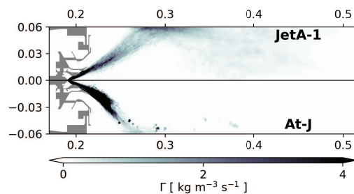
Fig. 5: Comparison of the time-averaged field of total evaporation rate in the midplane for both fuels.
