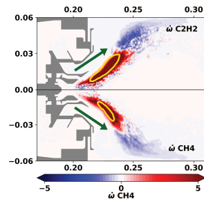
Fig. 13: Time averaged fields in the mid plane of the production and consumption rates of pyrolysed components.
