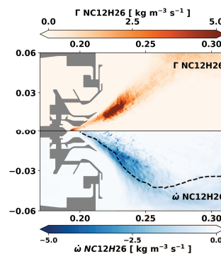
Fig. 10: Time-averaged evaporation (top) and consumption (bottom) zones of NC12H26.
