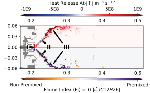
Fig. 12: Instantaneous heat release rate field (top) and Flame Index (bottom) for At-J.
