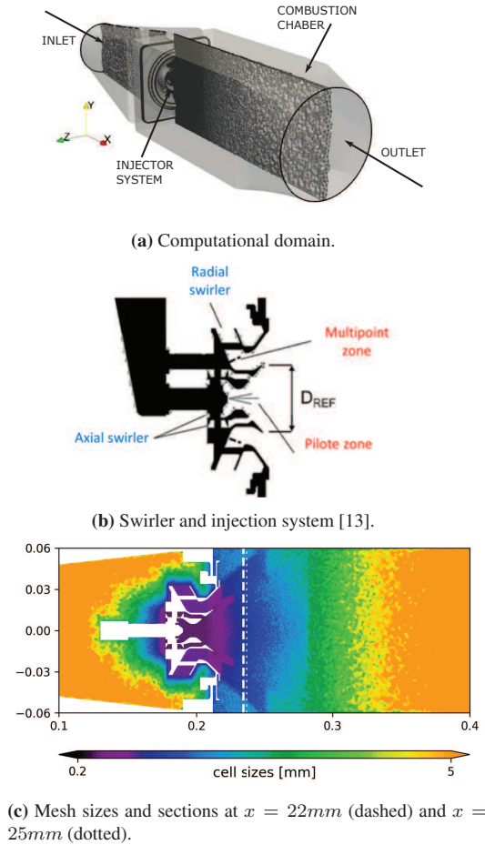
Fig. 1: Computational details of the setup.
