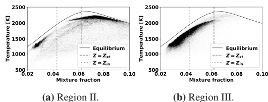
Fig. 14: Probability density plots in the temperature- mixture fraction space for the At-J flame.
