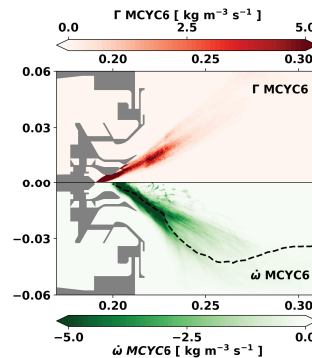
Fig. 9: Time-averaged evaporation (top) and consumption (bottom) zones of MCYC6.
