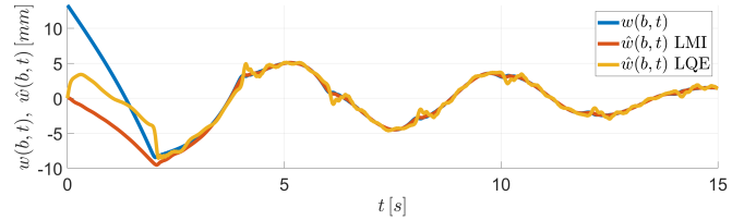
Fig. 2. w(b, t) is the end-tip displacement using the output feedback u(t) = -D_c y(t) . \hat{w}(b, t) is the observed end-tip position with L designed using LMI and LQE methods.
