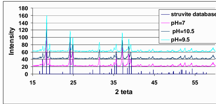
Figure 1. X- ray diffraction analysis results of formed precipitate from the synthetic solutions at different pH values and comparison with values from struvite database.
