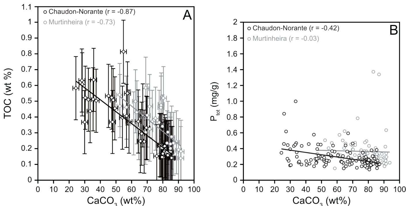
Figure 5 | (A) \text{CaCO}_3 (wt. %) versus TOC (wt. %) plot. (B) \text{CaCO}_3 (wt. %) versus P_{\text{tot}} (mg/g) plot. For both plots (A) and (B), Chaudon-Norante samples are in black and Murtinheira samples are in grey. There is a clear negative linear correlation between \text{CaCO}_3 and TOC values, with marlstones being more enriched in organic carbon. However, TOC values are low suggesting important effect of measurement uncertainties which are about 0.1 wt. % ( 1\sigma ). There is no relationship between \text{CaCO}_3 and P_{\text{tot}} values at Murtinheira, whereas a moderately good negative linear correlation is apparent for Chaudon-Norante, with marlstones being slightly enriched in P_{\text{tot}} .
