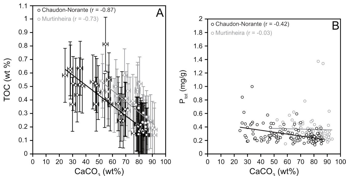
Figure 5 | (A) \text{CaCO}_3 (wt. %) versus TOC (wt. %) plot. (B) \text{CaCO}_3 (wt. %) versus P_{\text{tot}} (mg/g) plot. For both plots (A) and (B), Chaudon-Norante samples are in black and Murtinheira samples are in grey. There is a clear negative linear correlation between \text{CaCO}_3 and TOC values, with marlstones being more enriched in organic carbon. However, TOC values are low suggesting important effect of measurement uncertainties which are about 0.1 wt. % ( 1\sigma ). There is no relationship between \text{CaCO}_3 and P_{\text{tot}} values at Murtinheira, whereas a moderately good negative linear correlation is apparent for Chaudon-Norante, with marlstones being slightly enriched in P_{\text{tot}} .
