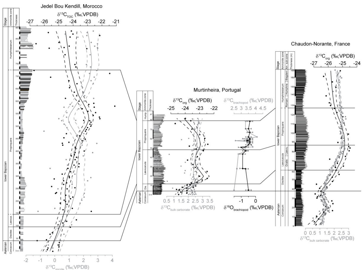
Fig. 8: \delta^{13}C_{bulk carbonate} (grey squares; labelled \delta^{13}C_{micrite} in Morocco following Bodin et al., 2017) versus \delta^{13}C_{org} (black circles; labelled \delta^{13}C_{TOC} in Morocco following Bodin et al., 2017) at Jedel Bou Kendill (Morocco; updated chronostratigraphic scheme in Bodin et al., 2020), Murtinheira (Portugal) and Chaudon-Norante (France) following a SW-NE transect. At Murtinheira, \delta^{13}C_{brachiopod} (‰, VPDB; grey squares) and \delta^{18}O_{brachiopod} (‰, VPDB; black circles) from Ferreira et al (2019) are plotted. The error bars for \delta^{18}O_{brachiopod} are \pm 2\sigma analytical uncertainty.
