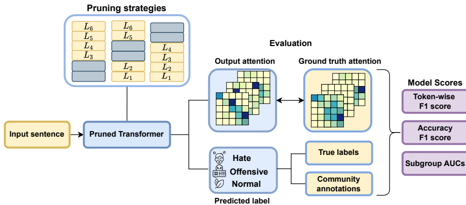
Fig. 1. End-to-end experimental pipeline. We prune the model by removing the layers, then use output attentions and predicted labels to evaluate Token F1 score, Accuracy/F1 scores, and Subgroup/BPSN/BNSP AUCs.
