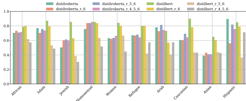
(b) DistilBERT/DistilRoBERTa
