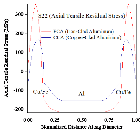
Fig 6. Axial tensile residual stress (S22) profile along the diameter (CCA vs FCA)
