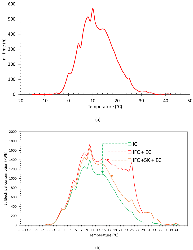
Fig. 9. (a) Temperature frequency in hours for the climatic data of Roubaix during 2018; (b) electrical consumption of the DC cooling system with respect to the external temperature of the DC in Roubaix for the three heat rejection systems: IFC + EC, IFC+5K + EC, and IC.
