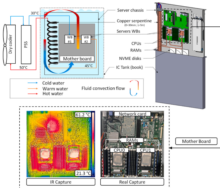
Fig. 2. Single-phase immersion/liquid-cooling technique architecture.
