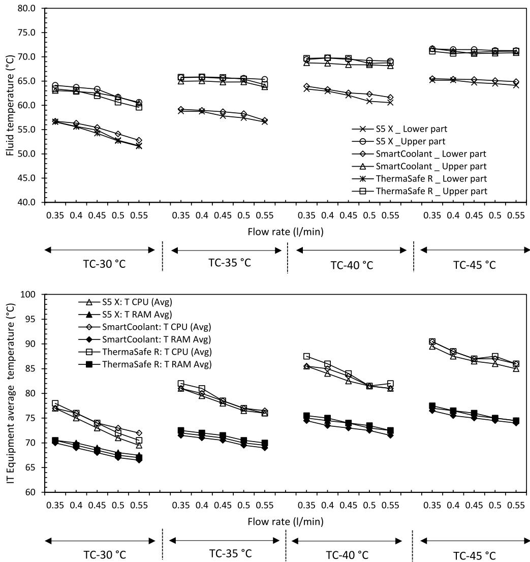
Fig. 5. Variations in (a) the IC fluid temperature and (b) the IT (CPUs and RAMs) temperatures, under different TCs and flow rates, using S5 X, SmartCoolant, and ThermaSafe R fluids.
