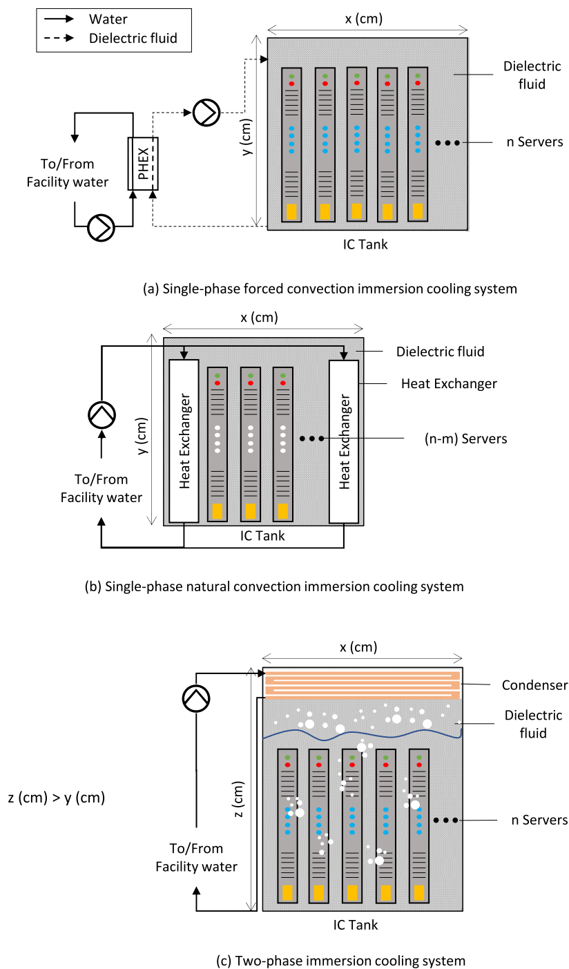
Fig. 1. Types of IC systems.
