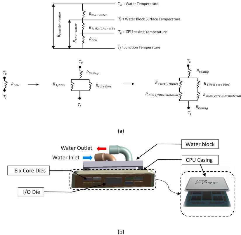
Fig. 10. (a) Electrical analogy for the heat transfer within the CPU junction point-water configuration, (b) AMD socket SP3 Processor and water block geometry view.
