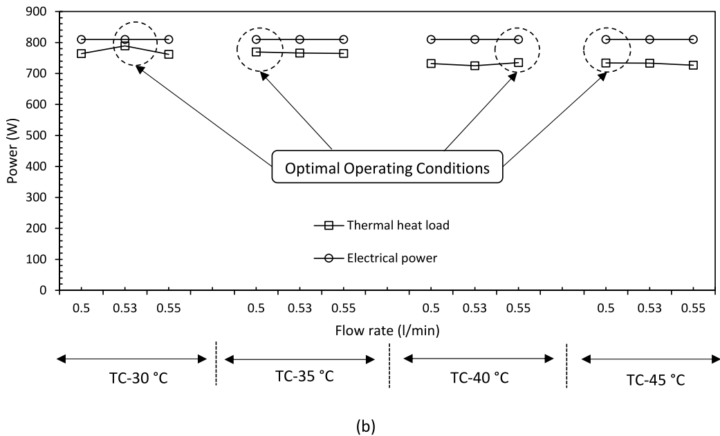
Fig. 8. IT electrical power and thermal heat load under different operating conditions for (a) Server #3 and (b) Server #4.
