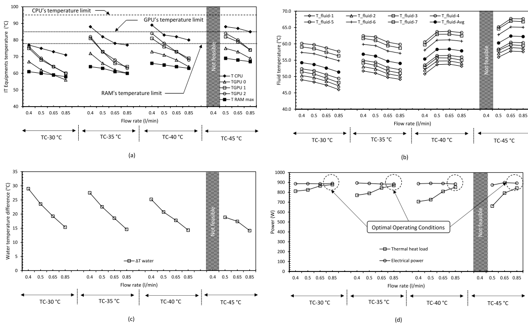
Fig. 7. Server #2: (a) IT equipment temperature, (b) IC fluid temperature, (c) water temperature difference, and (d) heat and IT power under different operating conditions.
