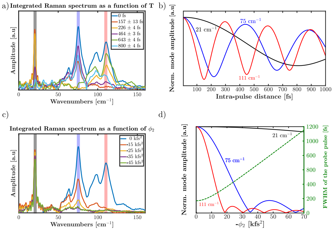
FIG. 3. (a) and (c) show the experimentally acquired spectra of CBZDH using the two-pulse probe structure and the chirped-probe structure respectively. In the two-pulse probe scheme (a) a spectral line disappears when intra-pulse distance T equals to an odd integer multiple of the half-period of the vibration mode. In the chirped-probe scheme (c) the higher wavenumber modes disappear when the probe pulse chirp is increased. The experimental results are in good agreement with the numerical estimation of the mode amplitudes using these two techniques (b) and (d). For instance comparing (a) and (b) it can be seen how the 111 \text{ cm}^{-1} mode goes undetected at T \approx 157 \text{ fs} , which is close to the half-period of this mode (which is 150 \text{ fs} ). Similarly comparing (c) and (d) it is seen that the 111 \text{ cm}^{-1} mode is undetected at \approx -15 \text{ kfs}^2 which broadens the pulse to \approx 300 \text{ fs} , which is the period of this mode.
