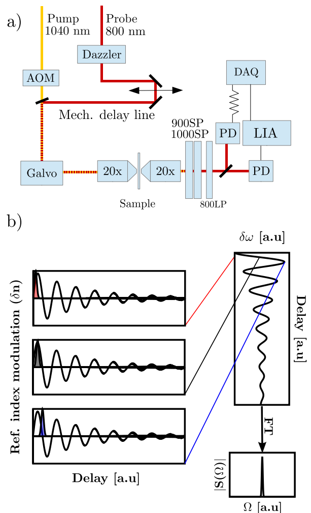
FIG. 1. a) The figure pictorially represents the key components of the setup. PD = photodiode, Galvo = galvanometric mirrors, AOM = acousto-optic modulator, DAQ = data acquisition card, LIA = lock-in amplifier SP = short pass, LP = long pass. b) The figure pictorially represents the logic of the spectral shift detection. The damped sinusoid represents the index variation in time due to the Raman oscillations. The Gaussian function represents the probe pulse field spectrum. Depending on the arrival time of the probe pulse with respect to the pump pulse, it sees a rising or falling edge of the refractive index which translates to a red or blue shift in the spectral centroid of the pulse [17] (indicated here by the color of the pulse). Allowing the probe pulse to pass through an edge filter centered at the probe central frequency, this spectral shift is converted to an intensity modulation in time, the Fourier transform of which gives the vibrational spectrum.
