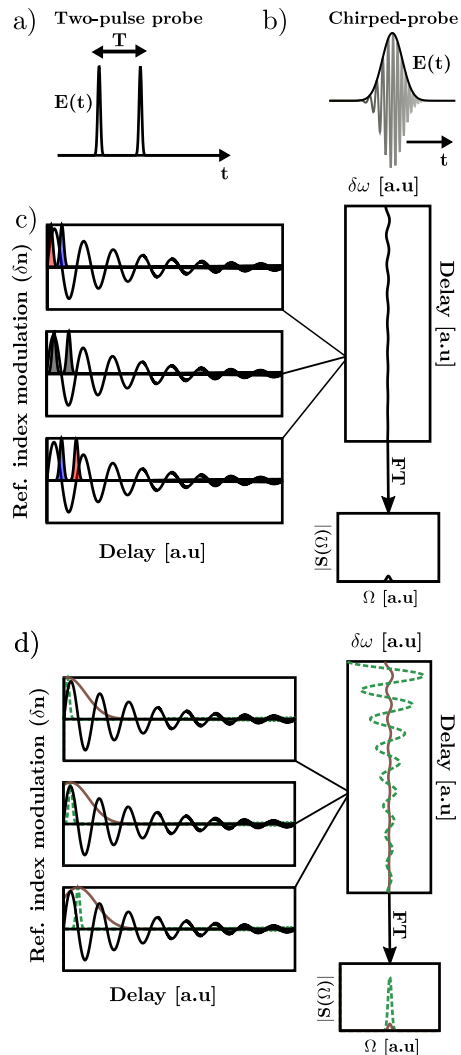
FIG. 2. a) and b) pictorially represent the two-pulse probe structure and the chirped-probe structure arriving with a varying delay after a transform-limited excitation pump pulse has excited the vibrational coherence in the sample. c) When the intra-probe pulse distance is equal to an odd integer multiple of half the vibrational period, the redshift experienced by one pulse compensates the blue shift experienced by the other pulse (indicated by the color of the pulse), thereby inhibiting the detection of the mode via spectral shift detection. d) The Gaussian functions represent the probe field amplitudes of a transform-limited probe pulse (the dashed green) and a chirped pulse (the solid brown). It is seen that with a transform-limited probe pulse, whose period is shorter than the period of the mode, the spectrum of the mode is well retrieved. As the pulse is chirped, the pulse gets broader in time and eventually surpasses the mode period. When this happens the interference between the input and the scattered fields evolve in such a way that the spectral centroid shift goes down and makes the Raman line disappear in the spectrum.
