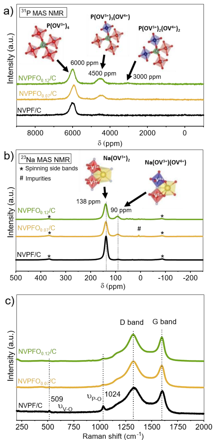
Figure 2: a) ^{31}P MAS NMR spectra of Na_3V_2(PO_4)_2F_{3-\gamma}O_\gamma/C phases ( \gamma = 0, 0.07 and 0.12 ) recorded at B_0 = 2.35 T with a 30 kHz MAS spinning frequency. PO_4 groups are represented as green tetrahedra, V^{3+} and V^{4+} octahedral units in red and blue, respectively. b) ^{23}Na MAS NMR spectra of Na_3V_2(PO_4)_2F_{3-\gamma}O_\gamma/C phases recorded at B_0 = 11.7 T with a 30 kHz MAS spinning frequency. c) Raman spectra of Na_3V_2(PO_4)_2F_{3-\gamma}O_\gamma/C phases
