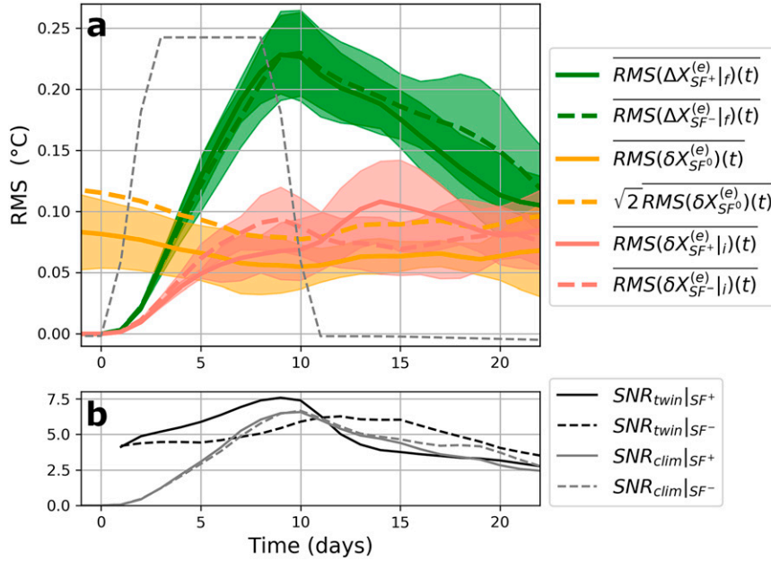
FIG. 3. (a) Time series of the ensemble averages of spatial RMS for various quantities computed for X = SST ; see text in section 2e and Eq. (7). The gray dashed line represents the amplitude modulation of the synoptic anomaly f(t) . (b) Signal-to-noise ratios (SNR) as defined in section 2e.
