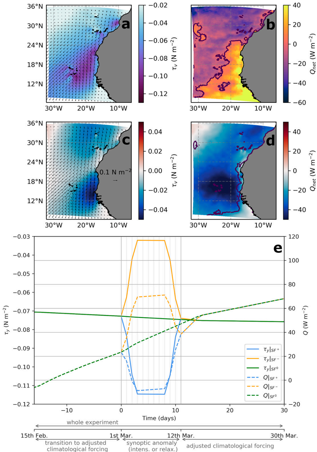
FIG. 2. Canary Current (a),(c) meridional wind stress and (b),(d) net heat fluxes climatological (SF 0 ) fields in (a) and (b) and SF + anomaly fields in (c) and (d) at the peak of the synoptic intensification. Anomalies for SF - are the opposite of those for SF + . (e) The experimental timeline. Continuous (resp. dashed) lines indicate the evolution of the meridional wind stress (resp. net heat flux) averaged over the SSUS. Green (resp. blue and orange) lines are for climatological (resp. wind intensification and relaxation) forcings. A slight deviation from perfect SF + -SF - symmetry can be seen for heat fluxes, due at a small error. Its impact on simulated upper-ocean temperature is negligible (see section 2c).
