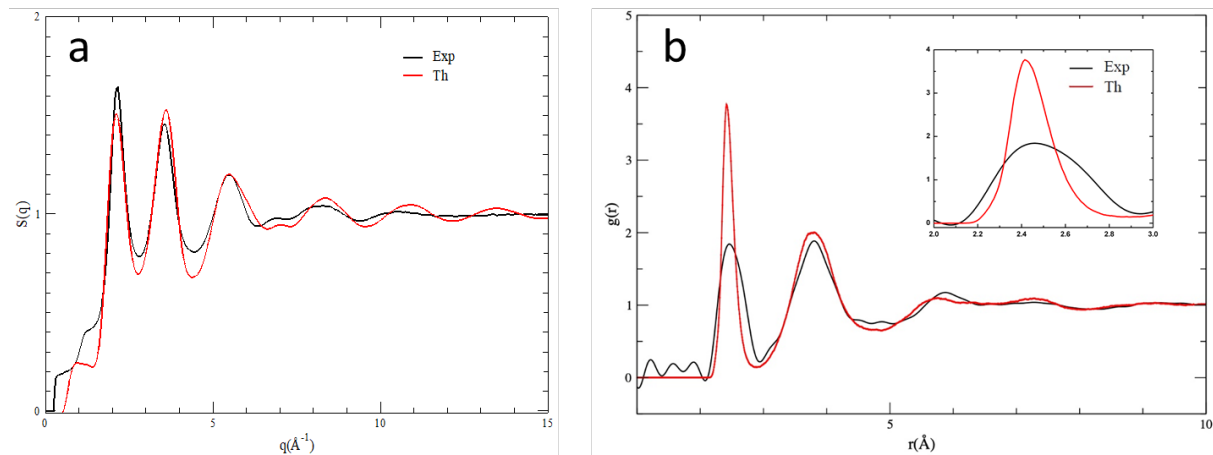
Figure 5. (a) Total neutron structure factors S(q) and (b) total pair correlation functions g(r) for \text{Ga}_8\text{Sb}_{27}\text{Se}_{65} glass composition. Experimental and theoretical data are in black and red, respectively. The inset graph emphasizes on the r -range between 2 and 3 \text{\AA} .
