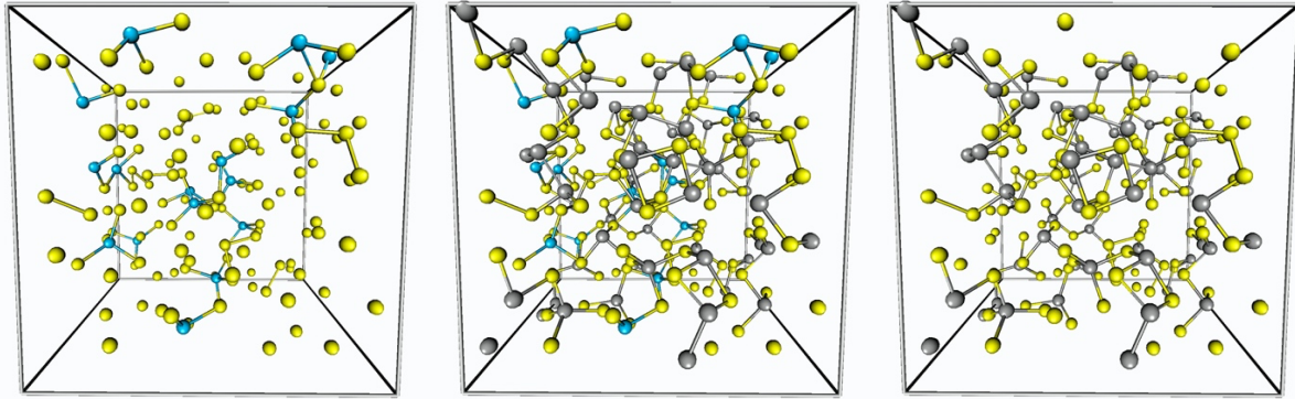
Figure 4. Visualization of \text{Ga}_8\text{Sb}_{27}\text{Se}_{65} glass (middle), Sb (grey), Se (yellow), Ga (cyan), together with two views in which Sb (left) and Ga (right) are discarded for the sake of clarity.
