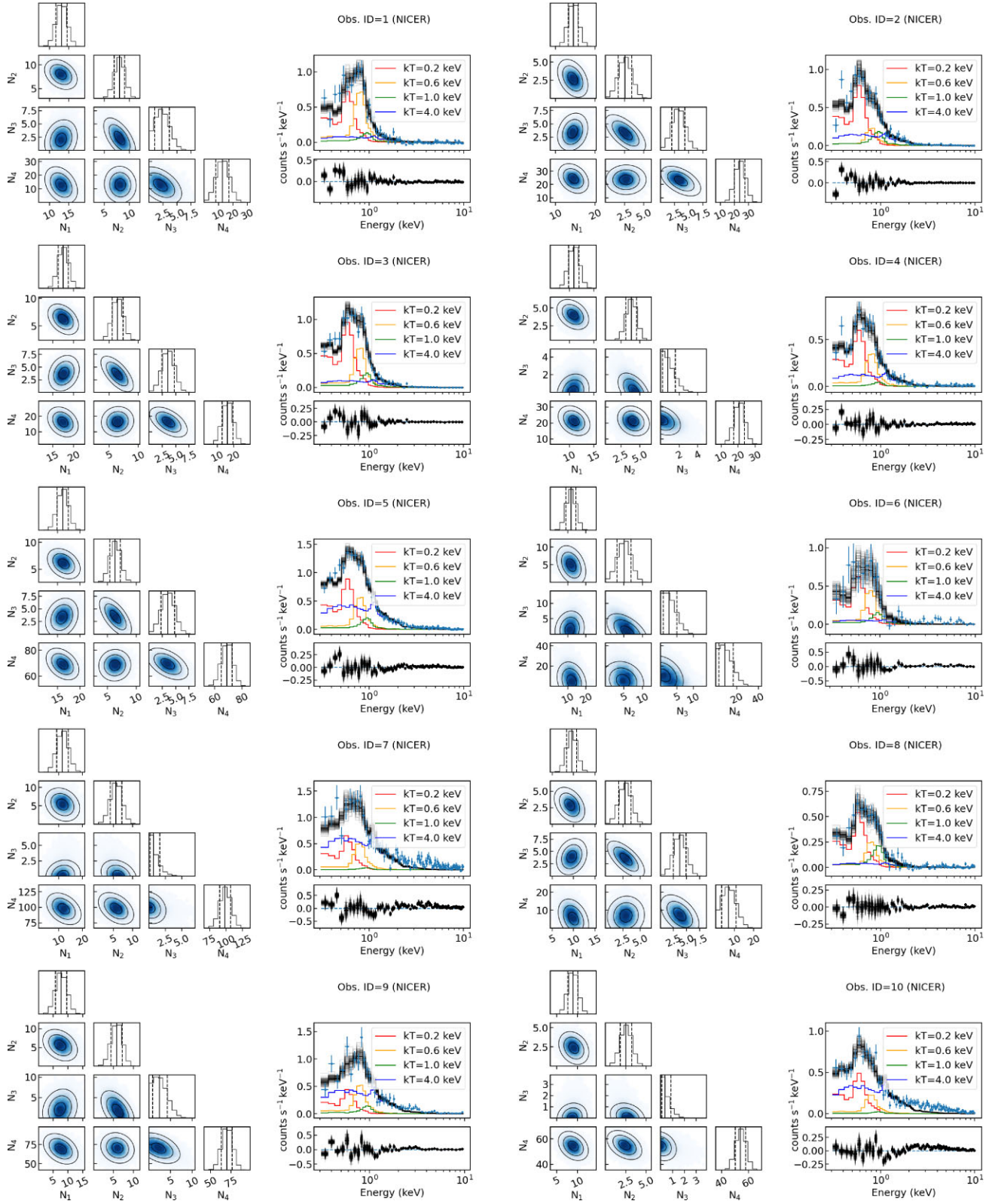
Figure B3. Spectral analysis of individual observations. The model fitted is the 4T model with n_{\text{H}} fixed at 0.03 \times 10^{22} \text{ cm}^{-2} . The Obs. IDs correspond to the IDs listed in Table 1. The solid vertical lines on the histograms mark the median values, and the vertical dashed lines mark the 68 per cent confidence intervals. N_i ( i = 1, 2, 3, 4 ) are proportional to the norms at 0.2 keV, 0.6 keV, 1.0 keV, and 4.0 keV, respectively, with N_i = \text{Norm}_i \times 10^5 . See Section 6.2 for details.
