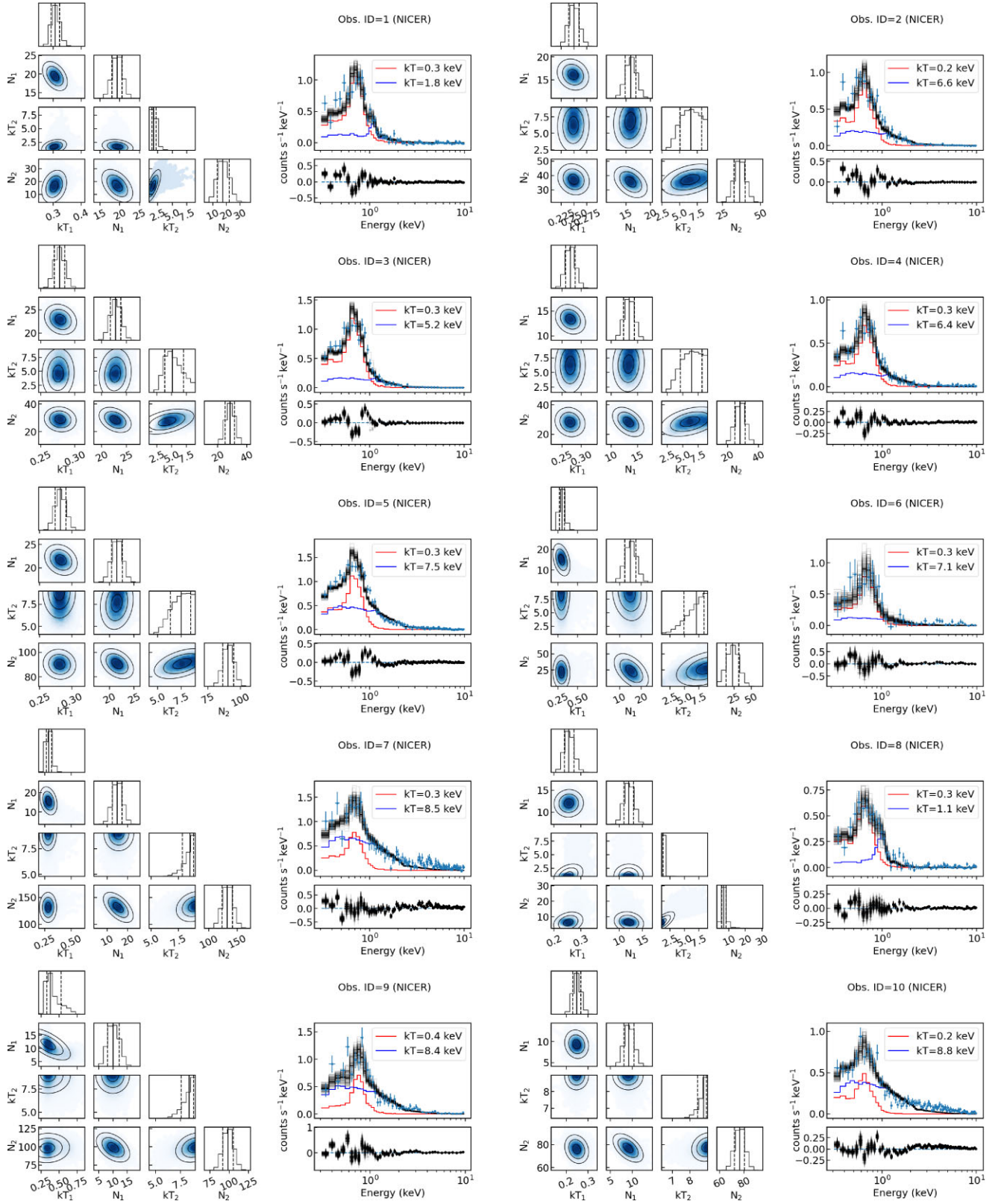
Figure B2. Spectral analysis of individual observations for the 2T model with n_{\text{H}} fixed at 0.03 \times 10^{22} \text{ cm}^{-2} . The Obs. IDs correspond to the IDs listed in Table 1. The solid vertical lines on the histograms mark the median values, and the vertical dashed lines mark the 68 per cent confidence intervals. N_i s ( i = 1, 2 ) are proportional to the norms at the two plasma temperatures given by kT_1 and kT_2 , respectively, with N_i = \text{Norm}_i \times 10^5 . See Appendix A for details.
