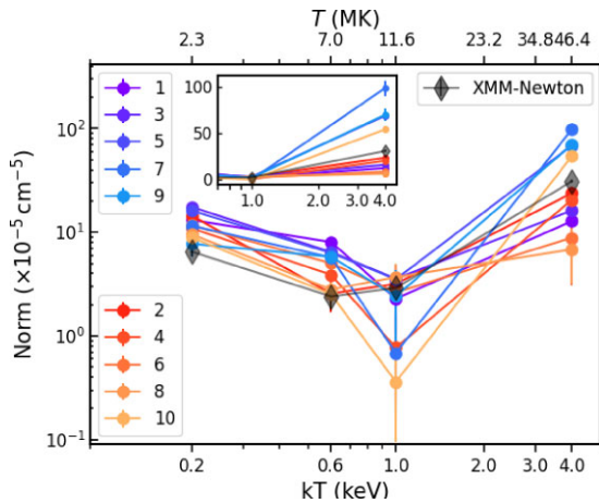
Figure 6. The normalization factors as a function of temperature (expressed in keV here) for the 4T model with n_{\text{H}} fixed at 0.03 \times 10^{22} \text{ cm}^{-2} . The error bars in the normalization factors correspond to 68 per cent confidence intervals ( 1\sigma ). The observations labelled with odd numbers correspond to periastron observations, and those labelled with even numbers correspond to out-of-periastron observations. The black diamonds represent the result obtained by Nazé et al. (2014) using the XMM-Newton observations. In the inset, we zoom over the region between 0.6 and 4 keV to show the difference between the normalization factors at the highest temperature (4 keV) for the different observations. Note that we have used a linear scale on the y-axis to make the difference more apparent.
