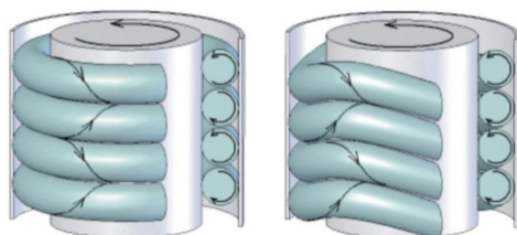
Figure 3. Taylor cells (Left-hand) and Wavy Taylor cell (Right-hand) [39].
