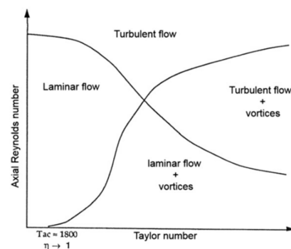
Figure 4. Flow regimes as a function of axial Reynolds number and Taylor number [41].
