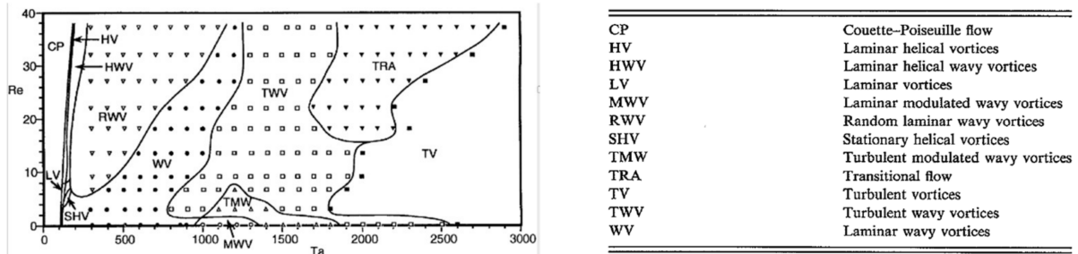
Figure 5. Different transitions of the Taylor–Couette–Poiseuille flow [41].
