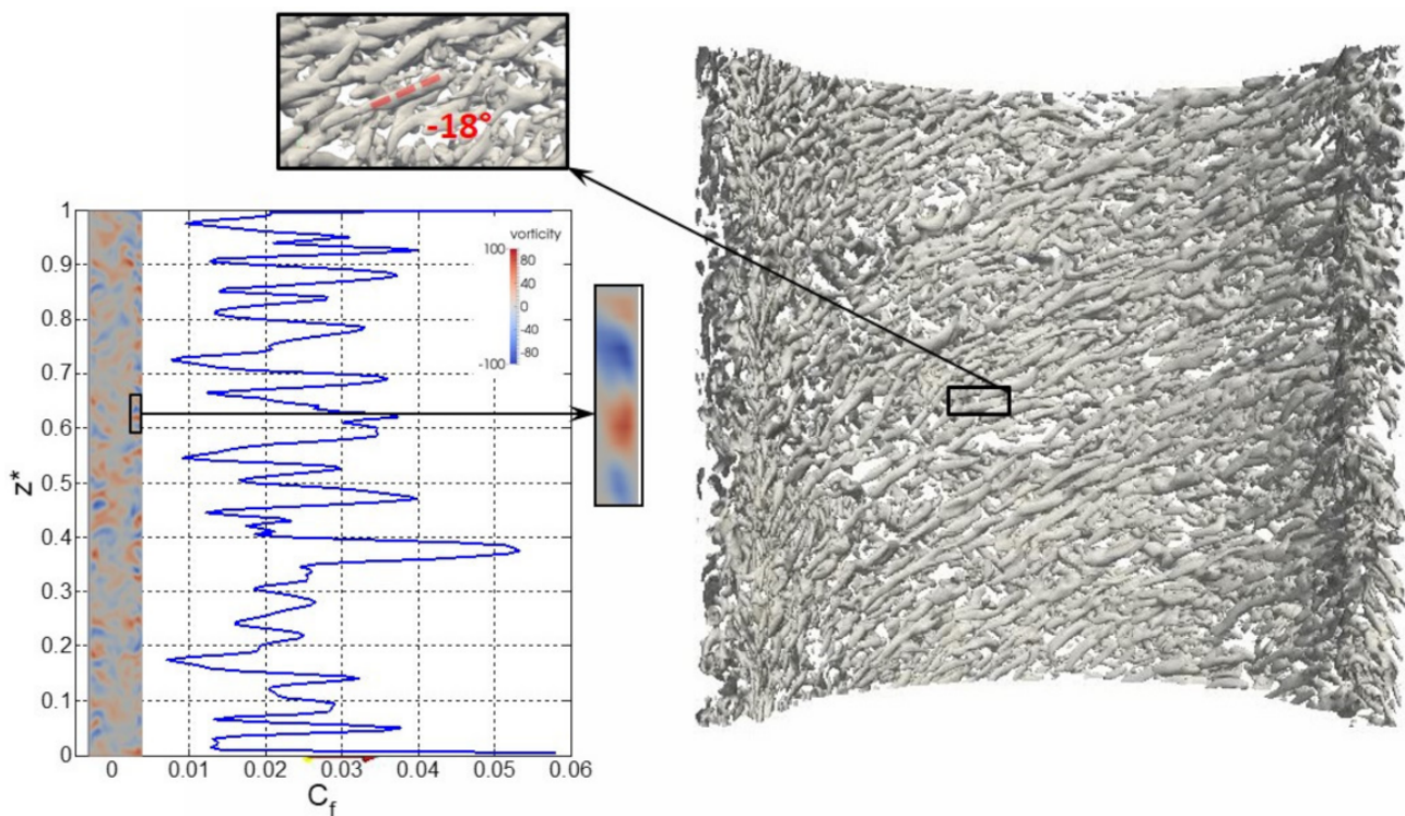
Figure 7. Simulation LES in the near-wall region of a Taylor–Couette–Poiseuille flow. Q-criterion applied for angular assessment of the vortex [41].
