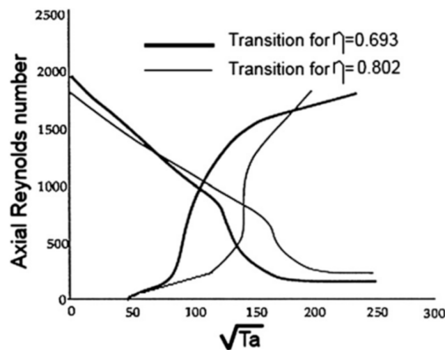
Figure 6. Taylor and axial Reynolds number flow transition: Influence of annulus thickness [41].
