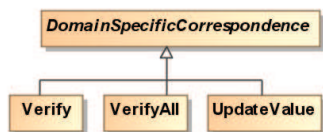
Figure 9: Extract of the specific part of the MMC meta-model for BTS domain
