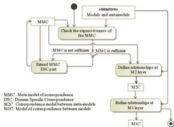
Figure 8 : The whole matching process
