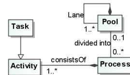
Figure 5: Extract of the BPMN meta-model
