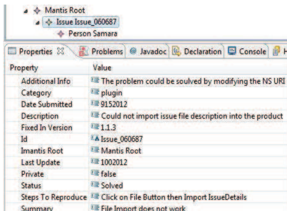
Figure 4: Snapshot of the BTS Mantis model
