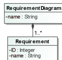
Figure 1 : Extract of the SysML meta-model
