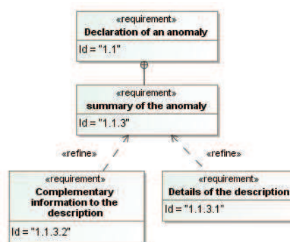
Figure 2: Snapshot of the BTS requirement model
