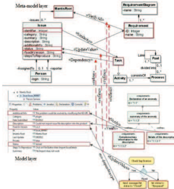
Figure 10: Examples of HLR & LLR relationships from BTS modelling
