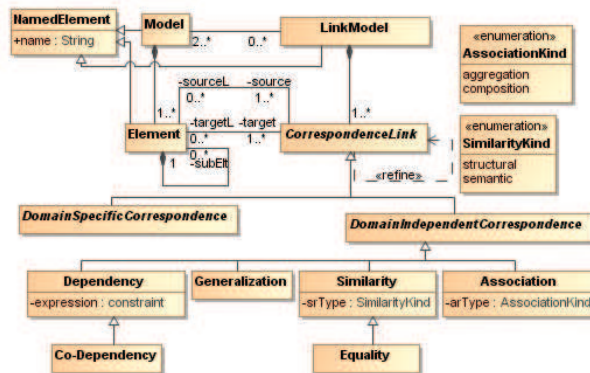
Figure 7: Overview of the MMC correspondence meta-model (generic part)
