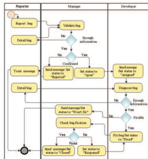
Figure 6: Snapshot of the BTS BPMN model
