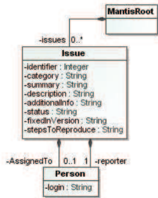
Figure 3 : Extract of the Mantis meta-model
