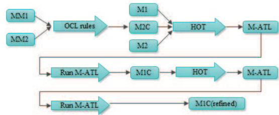
Figure 11: Process of model matching
