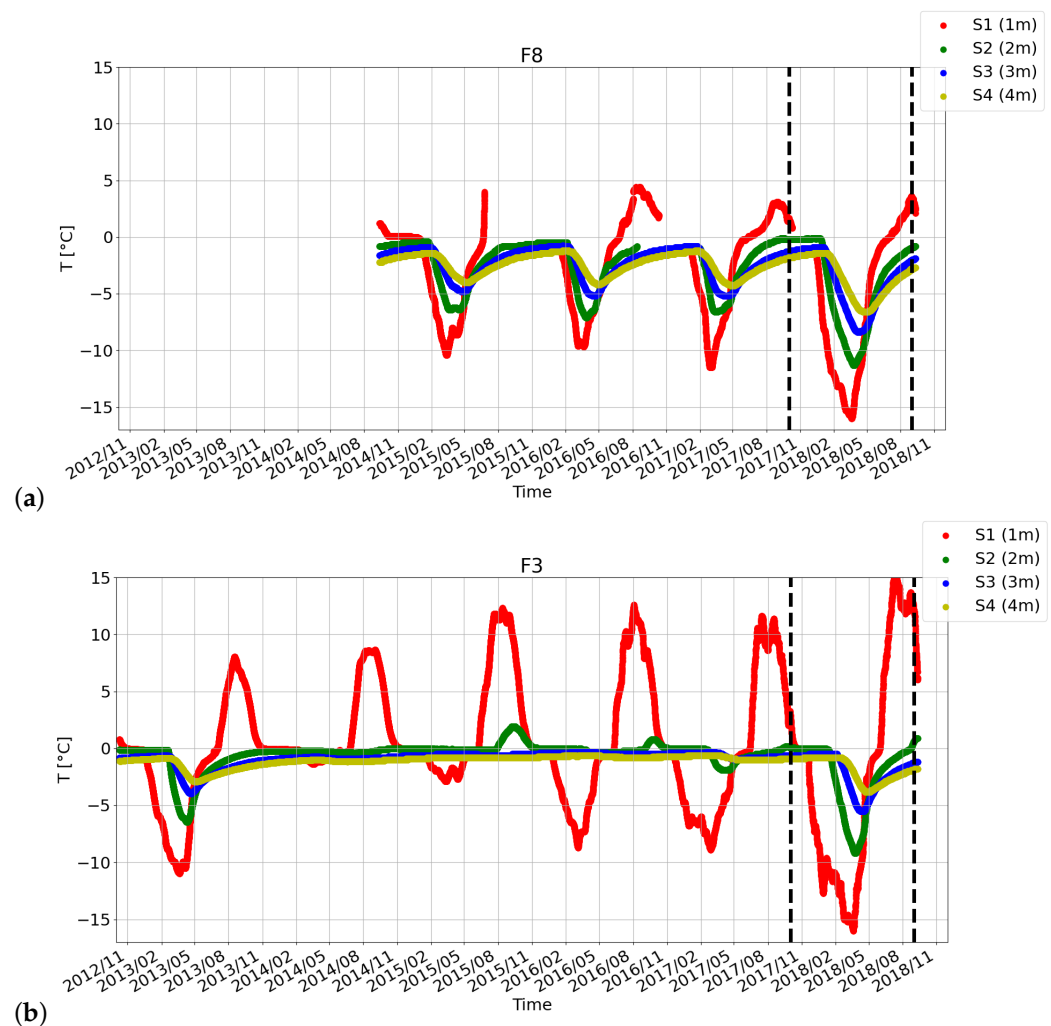
Figure 4. Time series acquired at four monitoring depths (sensor S1 at 1m depth, sensor S2 at 2 m depth, sensor S3 at 3 m depth, and sensor S4 at 4 m depth ) at two positions on CS1, (a) F8 left bank and (b) F3 in the riverbed (see Figure 3a for borehole positions). Dashed vertical black lines indicate the time of the geophysical surveys.
