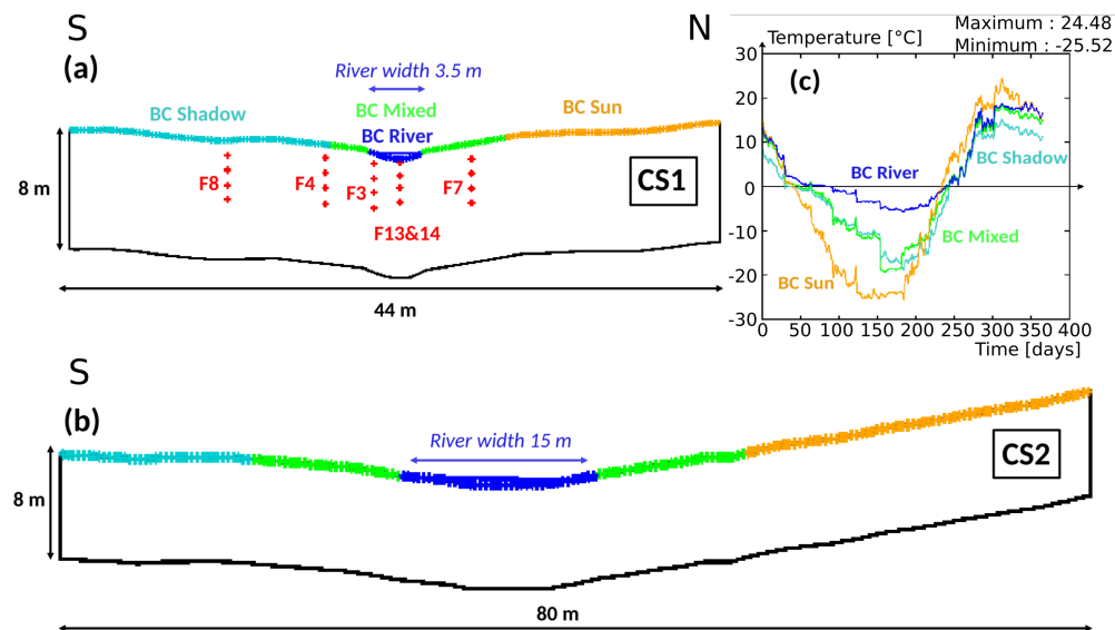
Figure 3. Modeled domain geometries for (a) CS1 and (b) CS2, including temperature measurement network (red crosses) and classification for surface temperature boundary conditions (BC) for four zones (river, shaded zone, mixed zone, sunny zone), and (c) the associated one year daily temperature time-series averaged over the available seven years of monitoring data, serving as model boundary conditions.
