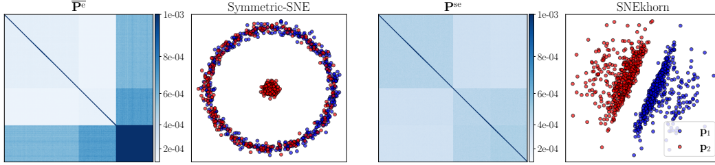
Figure 5: From left to right: entries of \overline{\mathbf{P}}^e (Symmetric-SNE) and associated embeddings generated using \overline{\mathbf{P}}^e . Then \mathbf{P}^{\text{se}} (SEA) matrix and associated SNEkhorn embeddings. Perplexity \xi = 30 .
