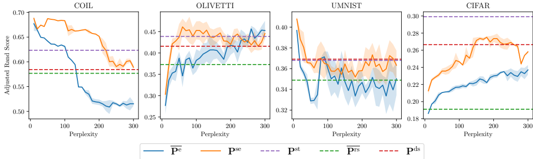
Figure 6: ARI spectral clustering score as a function of the perplexity parameter for image datasets.
