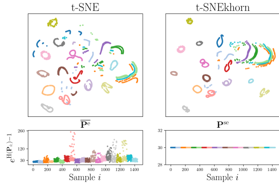
Figure 1: Top: COIL [34] embeddings with silhouette scores produced by t-SNE and t-SNEkhorn (our method introduced in Section 4) for \xi = 30 . Bottom: e^{H(\mathbf{P}_{i\cdot}^e)-1} ( perplexity ) for each point i .
