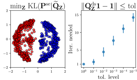
Figure 4: Left: SNEkhorn embedding on the simulated data of Section 5 using \tilde{\mathbf{Q}}_{\mathbf{Z}} instead of \mathbf{Q}_{\mathbf{Z}}^{ds} with \xi = 30 . Right: number of iterations needed to achieve \|\mathbf{Q}_{\mathbf{Z}}^{ds} \mathbf{1} - \mathbf{1}\|_{\infty} \leq \text{tol} with (Sinkhorn).
