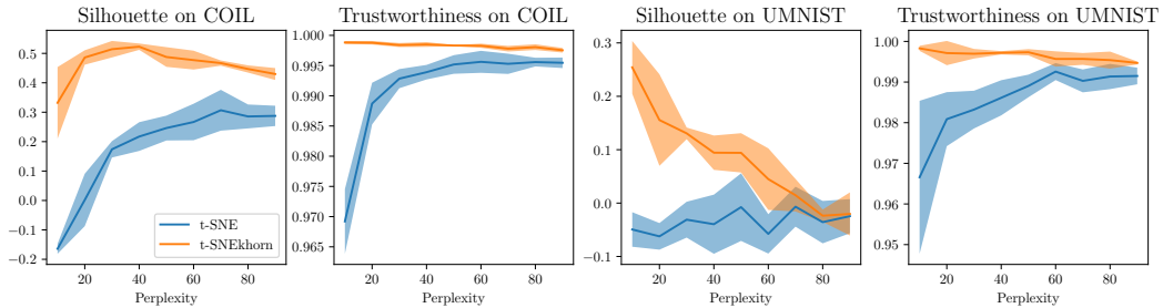
Figure 8: Dimensionality reduction scores as a function of the perplexity parameter.
