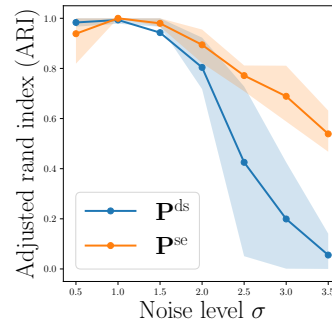
Figure 3: ARI spectral clustering on the example of three Gaussian clusters with variances: \sigma^2 , 2\sigma^2 and 3\sigma^2 (as in Figure 2).
