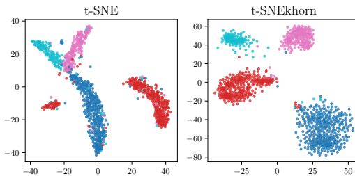
Figure 7: SNAREseq embeddings produced by t-SNE and t-SNEkhorn with \xi = 50 .
