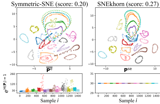
Figure 1: Top: COIL [37] embeddings with silhouette scores produced by Symmetric-SNE and SNEkhorn (our method introduced in Section 4) for \xi = 30 . Bottom: e^{H(\mathbf{P}_{i \cdot}^e)-1} ( perplexity ) for each point i .
