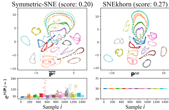
Figure 1: Top: COIL [37] embeddings with silhouette scores produced by Symmetric-SNE and SNEkhorn (our method introduced in Section 4) for \xi = 30 . Bottom: e^{H(\mathbf{P}_{i\cdot}^e)-1} ( perplexity ) for each point i .
