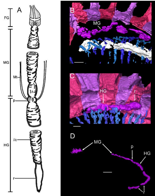
1298 1299 1300 Fig 9. Digestive system of extant and extinct diplopods. A: schematic illustration of a diplopod digestive tube 1301 (Fontanetti et al. 2015). B-C: Digestive tubes of Amynilyspes fatimae . (B) MNHN.F.SOT.2134. (C) 1302 MNHN.F.SOT.2129. (D) Digestive tube of Blanziulus parriati , specimen MNHN.F.SOT.81522. FG, foregut; HG, 1303 hindgut; i/c, ileo/colon; MG, midgut; Mt, Malpighian tubule; p, pylorus; r, rectum. Scale bars represent: 2 mm (D); 1 1304 mm (B); 500 \mu m (C). 1305 1306 1307 1308 1309 1310 1311 1312
