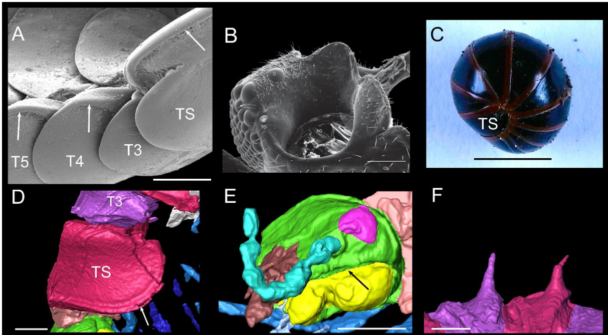
Fig 12. Morphological defences of pill millipedes. A-C: extant pill millipedes. (A) Details on margins of Glomeris guttata . (B) Antennal groove (antenna removed) of Cryxus ovalis (Linnaeus, 1758) (Sphaerotheriida), from Golovatch et al. 2012. (C) Glomeris marginata in volvation. D-F: Amynilyspes fatimae , specimen MNHN.F.SOT.2134. (D) Details on margins. (E) Details on the head. (F) Details on spines. AG, antennal groove; BR, brim of head; Cly, clypeus; IL, incisura lateralis; O, isolated ocellus; TO; organ of Tömösváry; TS, thoracic shield; T#, tergite number #. White arrows on (A) and (D) indicate margins. Black arrow on (E) indicate lateral ridge. Scale bars represent: 5 mm (C); 1 mm (D-F); 500 µm (A); 400 µm (B).
