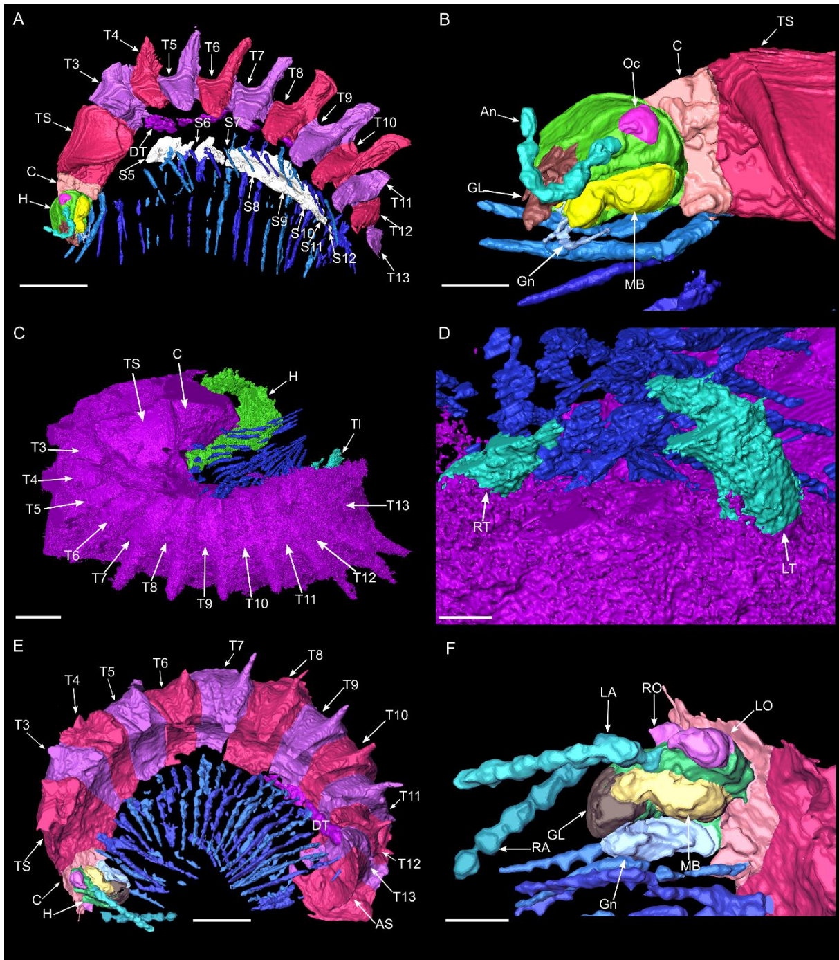
Fig 3. 3D reconstructions of Amynilyspes fatimae . A-B: Holotype MNHN.F.SOT.2134. (A) Left lateral view. (B) Details on the head. C-D: Paratype MNHN.F.SOT.14983. (C) Oblique postero-dorsal view. (D) Details on the telopods. E-F: Paratype MNHN.F.SOT.2129. (E) Left lateral view. (F) Details on the head. An, antenna; AS, anal shield; C, collum; DT, digestive tube; GL, gnathal lobe; Gn, gnathochilarium; H, head; LA, left antenna; LO, left ocular field; LT, left telopod; MB, mandibular base; Oc, ocular fields; RA, right antenna; RO, right ocular field; RT, right telopod; S#, sternite number #; T#, tergum number #. Scale bars represent: 3 mm (A); 2 mm (E); 1mm (B-C); 500 \mu m (F); 100 \mu m (D). The reconstructions of MNHN.F.SOT.14983 are made from the scans of the \mu CT SKyscan 1272. All the other reconstitutions are made from the scans of the Phoenix X-ray Phoenix v|tome|x CT-scan.
