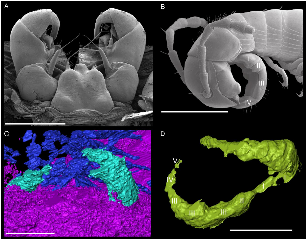
Fig 11. Sexual appendages of pill millipedes and Juliformia. (A) Outer telopods of Glomeris marginata (Glomerida). (B) Front part of Koiulus interruptus (Enghoff, Jensen & Mikhaljova, 2017) (Julida: Mongoliulidae), from Enghoff et al. 2017. (C) Inner telopods of Amynilyspes fatimae , specimen MNHN.F.SOT.14983. (D) Details on claspers of Blanziulus parriati , specimen MNHN.F.SOT.2113. Roman number #, corresponding clasper segment. Scale bars represent: 2 mm (D); 1 mm (A, C); 100 \mu m (B).
