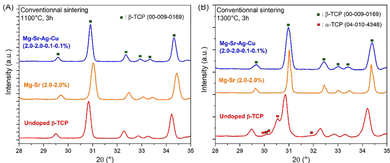
Figure 8. X-ray diffraction (XRD) patterns of sintered undoped and co-doped \beta -TCP pellets at (A) 1100°C for 3 h and (B) 1300°C for 3 h.
