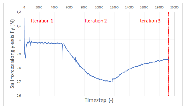
(f) Evolution of force along y-axis provided by the sails during the computation
