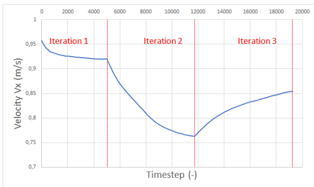
(c) Evolution of yacht's speed along x-axis during the computation
