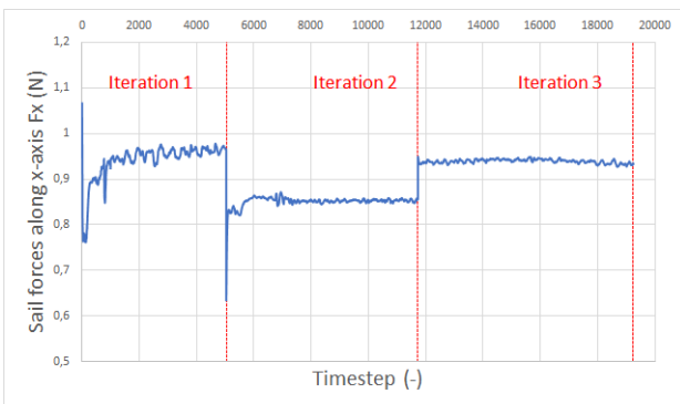
(e) Evolution of force along x-axis provided by the sails during the computation
