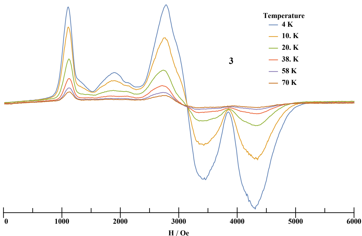
Figure S23. Evolution with the temperature of the X band EPR spectrum of 3 .
