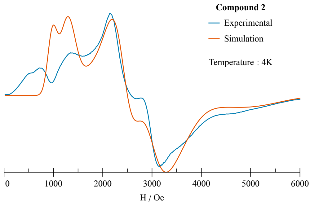
Figure S22 Experimental X band EPR spectrum of 2 at 4K and S=3/2 simulation obtained by least squares fitting using Easyspin Matlab toolbox ( D= 5.98 \text{ cm}^{-1} fixed, best parameters g_x=2.75 , g_y=2.03 , g_z=2.33 , E/D=0.296 )
