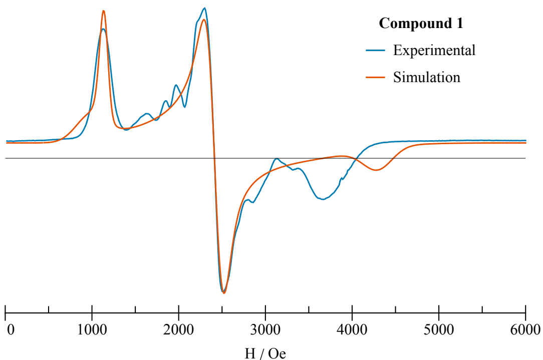
Figure S20. Experimental X band EPR spectrum of 1 at 4K and S=3/2 simulation obtained by least squares fitting using Easyspin Matlab toolbox ( D=4.6\text{ cm}^{-1} fixed, best parameters g_x=2.75 , g_y=2.12 , g_z=4.823 , E/D=1/3 \Gamma_x=747\text{ G} \Gamma_y=847\text{ G} , \Gamma_z=3827\text{ G} )
