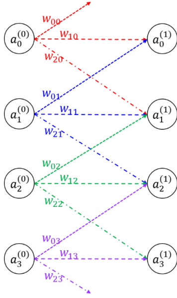
Fig. 2 Example of a simple OCNN with corresponding mathematical formula; a_i^{(l)} represents the i -th input or output node in the l -th layer; w_{ij} indicates the weight connecting the j -th input node and the i -th output node; b_i is the i -th bias; N_m is the number of weights connected to an input/output or the size of a kernel; \sigma is a sigmoid function
