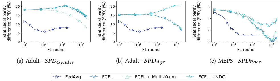
Fig. 4. Interaction between FL bias mitigation and FL robustness mechanisms
