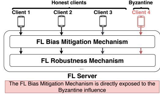
Fig. 2. Applying bias mitigation first in Byzantine setting does not work
