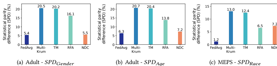
Fig. 3. Impact of FL robustness methods on Bias
