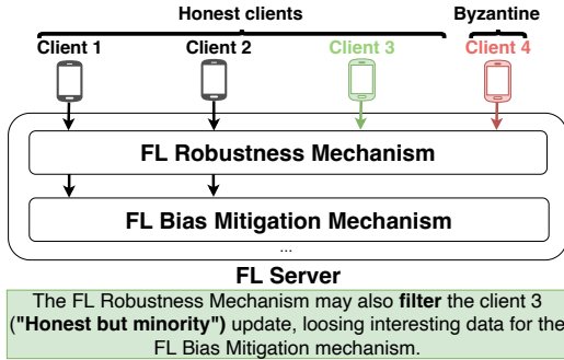
Fig. 1. Applying classical robust aggregators hinder FL bias mitigation
