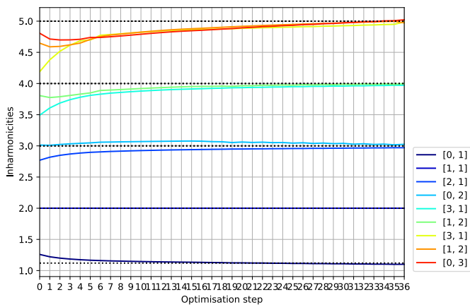
Figure 16: Evolution of inharmonicity of each mode relative to the mode (1, 1) during optimisation
