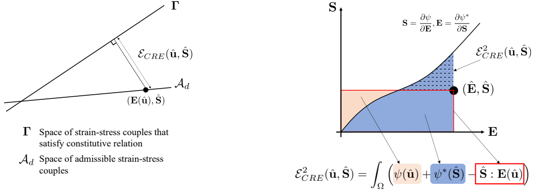
Figure 2: Left: interpretation of the CRE in the space of strain-stress couples. Right: interpretation of the CRE with the stress-strain curve.
