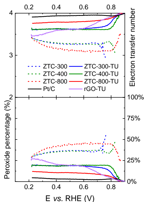
Figure 11. Number of electrons transferred per oxygen molecule (top) as well as fraction of peroxide formed during the reduction process (bottom). Calculations were done according to equations 2 and 3 using results shown in Figure 10a. Results obtained with Pt/C and rGO-TU materials are shown for comparison.
