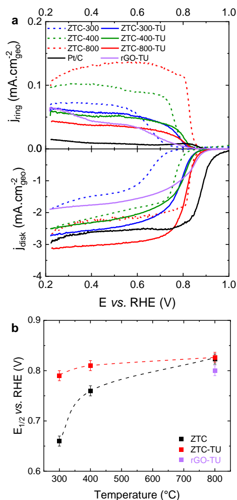
Figure 10. a) RRDE polarization curves recorded with all ZTC-based catalysts and Pt/C reference catalyst. b) Half-wave potential measured on polarization curves recorded in Figure a. The half-wave potential obtained with rGO-TU catalyst is shown for comparison.
