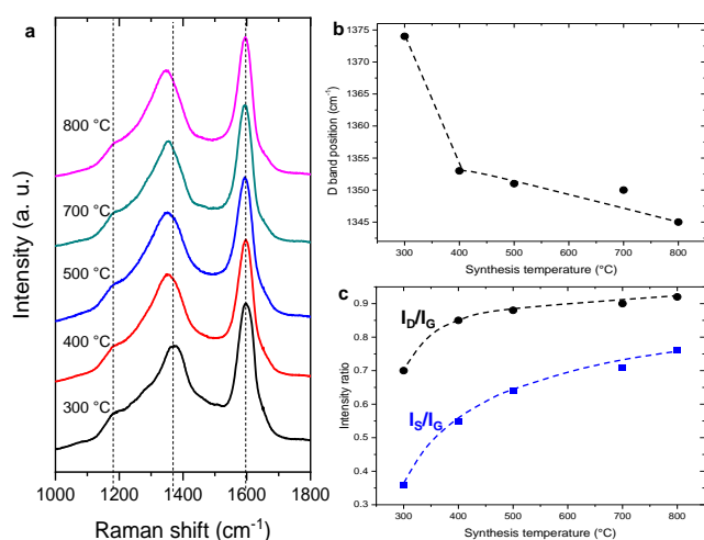
Figure 8. Raman spectra of materials synthesized at different synthesis temperatures (a). Raman D band position (b) and I_D/I_G and I_S/I_G intensity ratios as a function of the synthesis temperature (c). Color code: 300 ^{\circ}\text{C} (black), 400 ^{\circ}\text{C} (red), 500 ^{\circ}\text{C} (blue), 700 ^{\circ}\text{C} (green) and 800 ^{\circ}\text{C} (purple).
