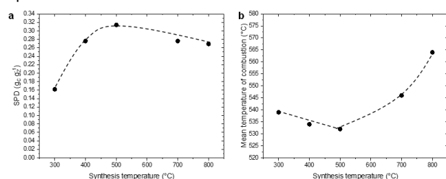
Figure 1. Evolution of SPD (a) and mean temperature of combustion (b) as a function of the synthesis temperature.
