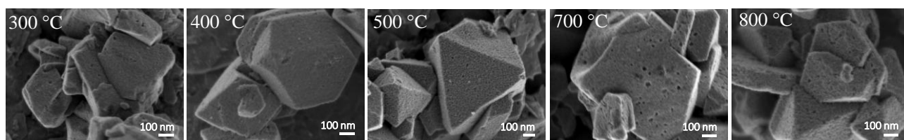
Figure 4. SEM images of ZTCs achieved at different synthesis temperatures.
