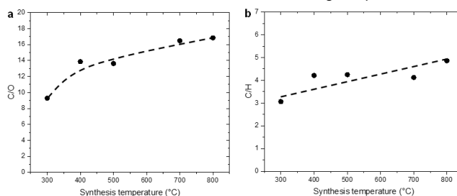
Figure 7. Atomic C/O (a) and C/H ratio (b) of ZTCs as a function of the synthesis temperature.
