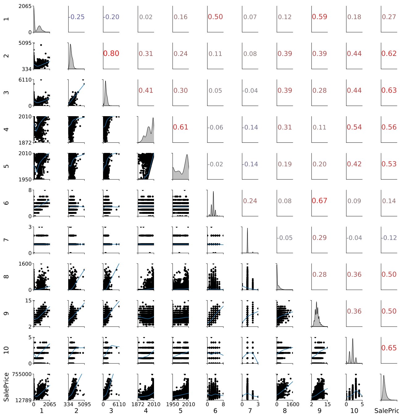
Figure 16: Data pairs plot for the Ames housing dataset providing: the variable histograms (diagonal), and for each variable pair the CC (upper panel), as well as scatter plots and fitted smoothers (lower panel).
