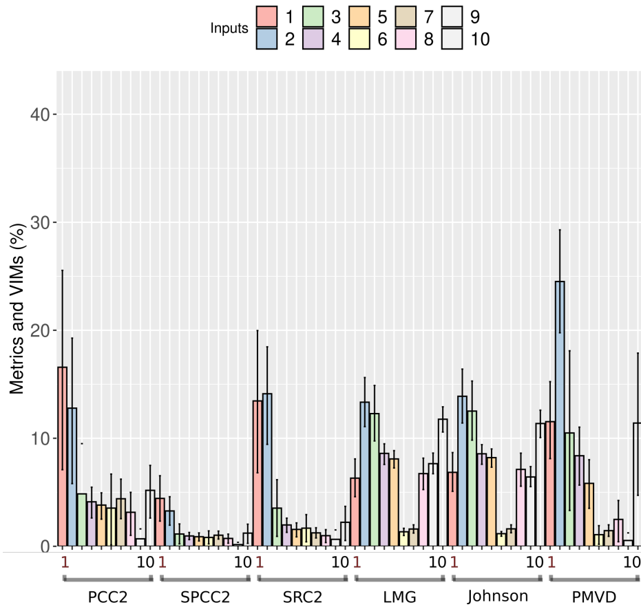
Figure 8: Estimates (with bootstrap) of the metrics (PCC 2 , SPCC 2 ) and the VIMs (SRC 2 , LMG, PMVD, Johnson) for the Ames housing data. Inputs are numbering by the following: SecondFlrSF (1). FirstFlrSF (2). TotalBsmSF (3). YearBuilt (4). YearRemodAdd (5). BedroomAbvGr (6). KitchenAbvGr (7). MasVnrArea (8) TotRmsAbvGrd (9) GarageCars (10).
