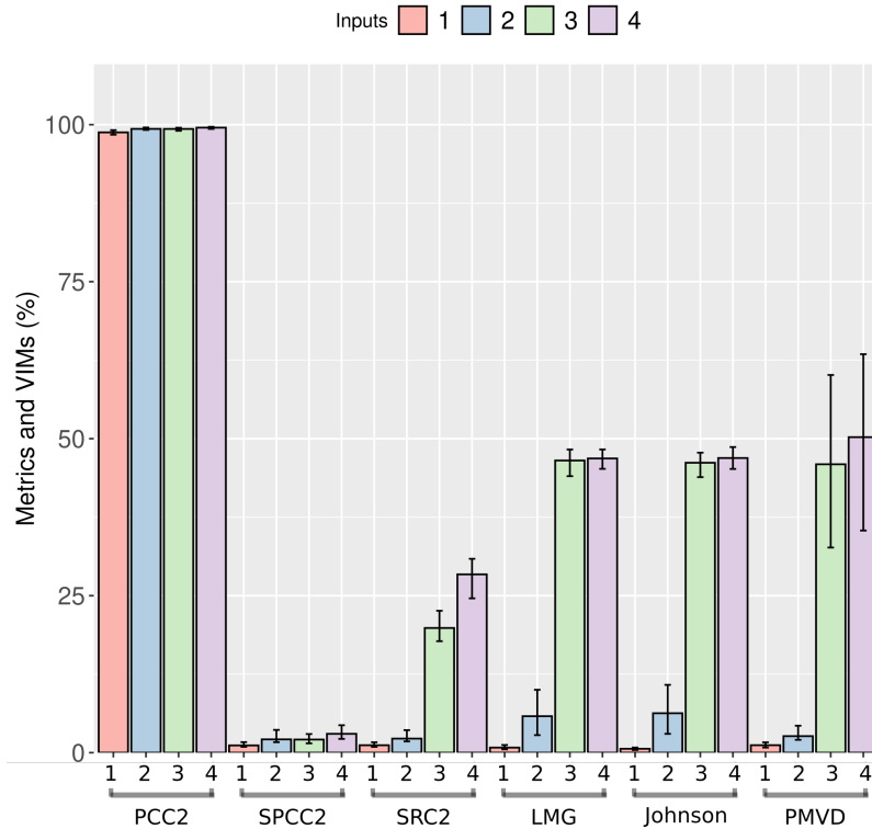
Figure 4: Estimates (with bootstrap) of the metrics ( PCC^2 , SPCC^2 ) and the VIMs ( SRC^2 , LMG, PMVD, Johnson) in the collinear case.
