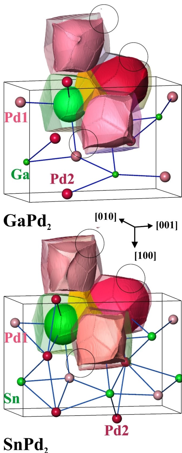
Figure 7. QTAIM atoms (transparent shapes) and ELI-D basins of the inner shells (pink and red basins) in \text{GaPd}_2 and \text{SnPd}_2 by formation of the four-atomic bonds \text{Ga-Pd2-Pd1-Pd1} and \text{Sn-Pd2-Pd1-Pd2} (orange bond basin, cf. Figure 4). For black circles, cf. text.
