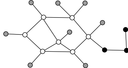
(b) A sputnik graph. The white vertices are part of cycles, the grey vertices are their antennas, and the black vertices do not belong to any cycle, nor are antennas.
