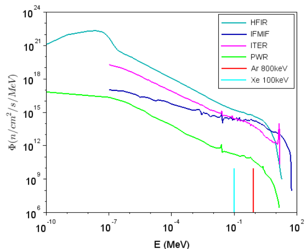
Figure 1: Neutron and ions spectra \phi for different nuclear reactors and ion beam facilities (pink line: ITER (fusion reactor), turquoise line: HFIR (High Flux Isotope Reactor), navy line: IFMIF (International Fusion Materials Irradiation Facility), green line: PWR (Power Water Reactor); red line: Ar 800 keV; blue line: Xe 100 keV)
