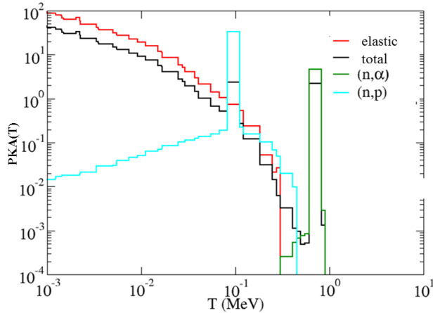
Figure 3: Comparison of PKA spectra as a function of the recoil energy T for different nuclear reactions occurring in the impinging of the ^{59}\text{Ni} isotope with a neutron (green line : (n, \alpha) nuclear reaction; blue line: (n, p) nuclear reaction; red line: elastic collision; black line: all processes are taken into account). All these calculations were performed for the HFIR reactor with the TENDL-2015 library on pure ^{59}\text{Ni} isotope.
