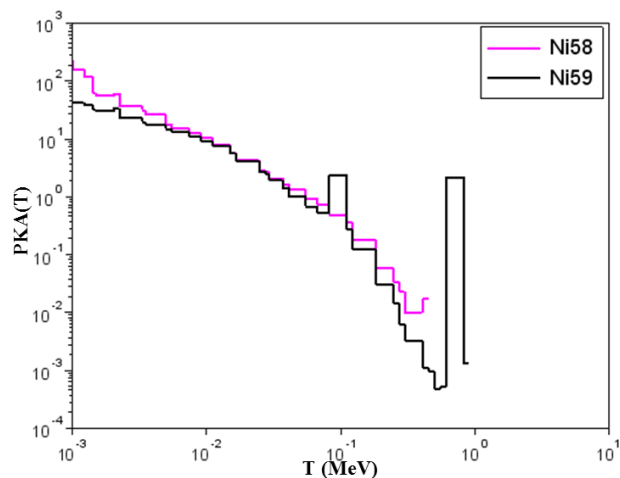
Figure 2: PKA spectra as a function of the energy of recoil atoms T in pure ^{58}\text{Ni} (magenta line) and ^{59}\text{Ni} (black line) isotopes. Two distinct peaks are clearly observed on the ^{59}\text{Ni} PKA distribution pointing out the impact of the Ni isotopes on the primary damage production. These calculations result from the integration of neutron-isotopes cross sections with the neutron spectrum of the HFIR facility. All these calculations were performed using the JENDL-4.0 library.
