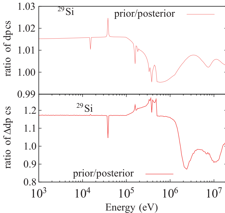
Fig. 27. Ratios of prior over posterior dpcs and dpcs uncertainties for ^{29}\text{Si} , taking into account the ^{\text{nat}}\text{Si} and \text{SiO}_2 experimental data.
