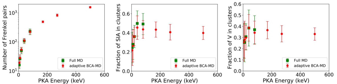
Fig. 41. Calculations developed so far up to 0.5 MeV PKA energy show the number of FPs, fraction of self-interstitial atoms (SIA), then vacancies in clusters as a function of PKA energy.
