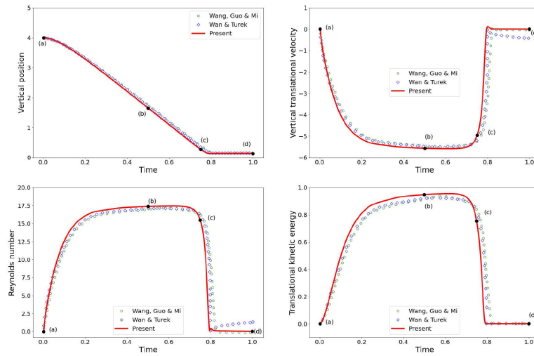
Figure 1: Evolution of the vertical position of mass center, vertical translational velocity, Reynolds number and translational kinetic energy. The red line are the present results, the green dotted and blue dotted lines correspond to results respectively taken from [19] and [18]. The streamlines and body position at four different time instants are represented.
