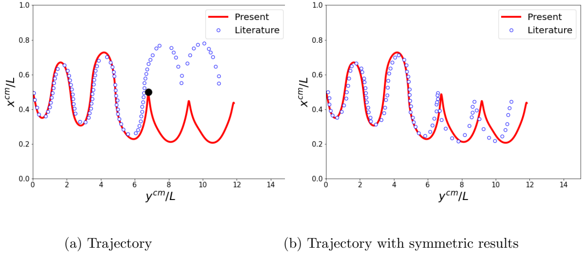
Figure 3: The left graph plots the trajectory of the ellipse center of mass. The red line corresponds to the present results and the blue dotted line represents the literature results [22]. The right graph shows the same trajectory but compares it to rotations happening on the other wall.
