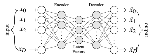
Fig. 1 Deep Autoencoder architecture.
