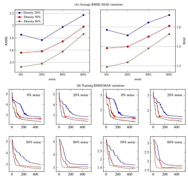
Fig. 7 The results with a training/testing set of ( density% )/(100 – density% ) for a clustered deep autoencoder prediction (on various noises and densities). (A) The average RMSE and MAE results, and (B) The training performance graph.
