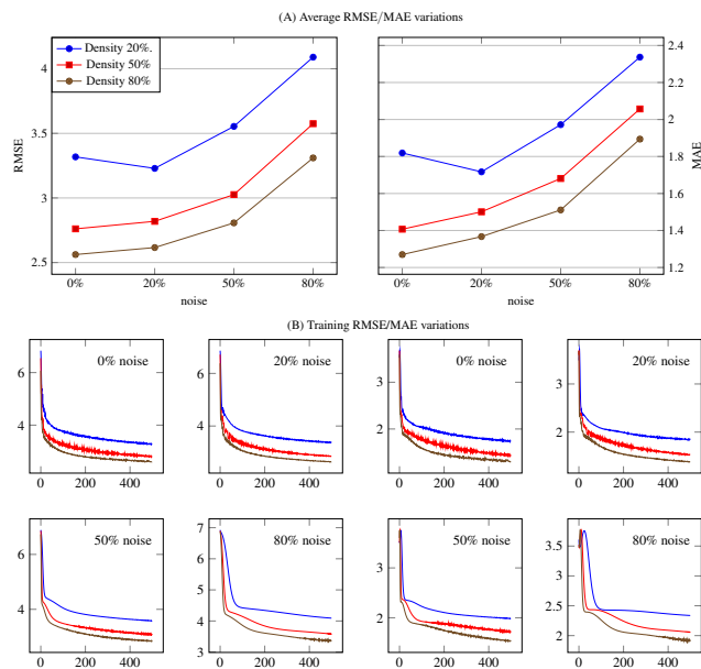
Fig. 6 The results with a training/testing set of ( density% )/(100 – density% ) for a deep autoencoder prediction (on various noises and densities). (A) The average RMSE and MAE results, and (B) The training performance graph.
