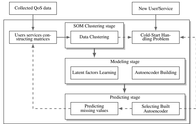
Fig. 3 Overview of the prediction system architecture
