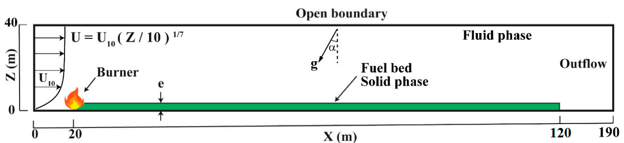
Figure 5. Computational domain and boundary conditions used in the 2D simulations.
