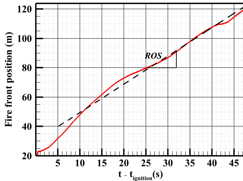
Figure 6. Variation with time of the furthestmost point of the pyrolysis front at the fuel bed surface obtained by FireStar2D after ignition time.
