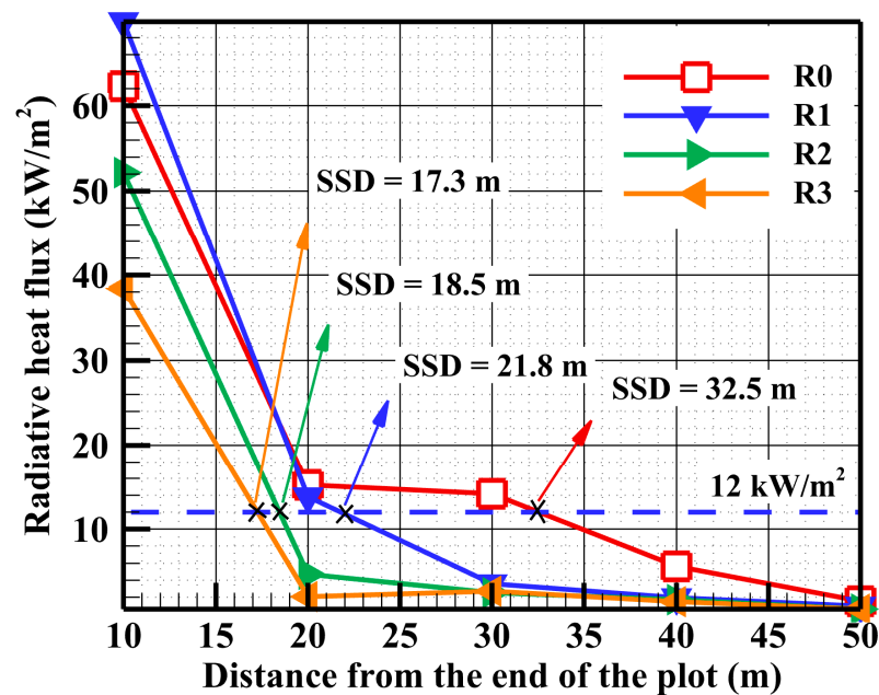
Figure 10. Variation of the radiative heat fluxes received by each level with respect to the distance separating the building from the fire front.
