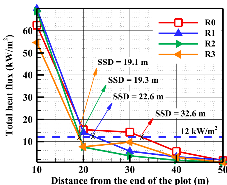
Figure 12. Variation of the total heat fluxes received by each level with respect to the distance separating the building from the fire front.
