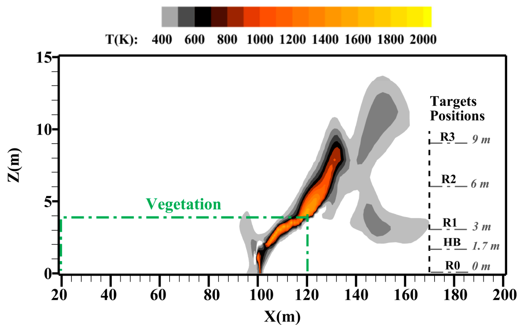
Figure 7. Instantaneous temperature field obtained using FireStar2D when the fire front reaches the end of the plot.
