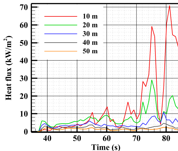
Figure 8. Variation with time of the radiative heat fluxes received by the human body at different positions ahead of the plot end.
