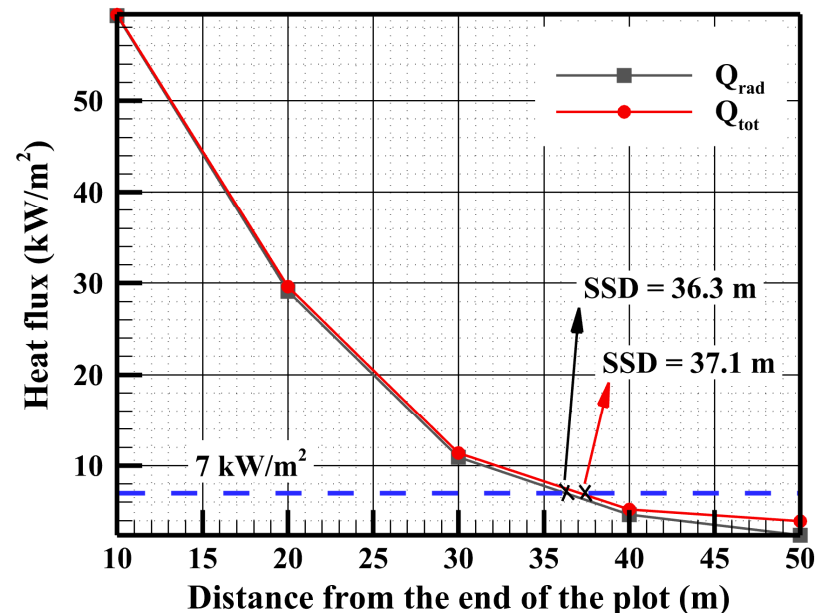
Figure 9. Maximum radiative heat fluxes received by the human body at different positions ahead of the fire front when the flames reach the end of the vegetation area.
