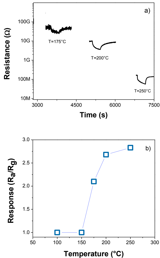
Fig. 5. a) Response at different temperature to 2500 ppm NO of the C-CDs sensor; b) trend of the sensor response vs. the temperature.
