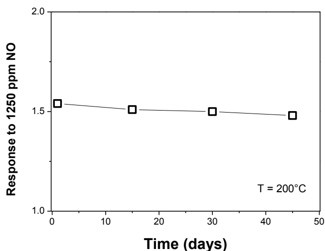
Fig. 8. Response of the C-CDs sensor registered at various times.
