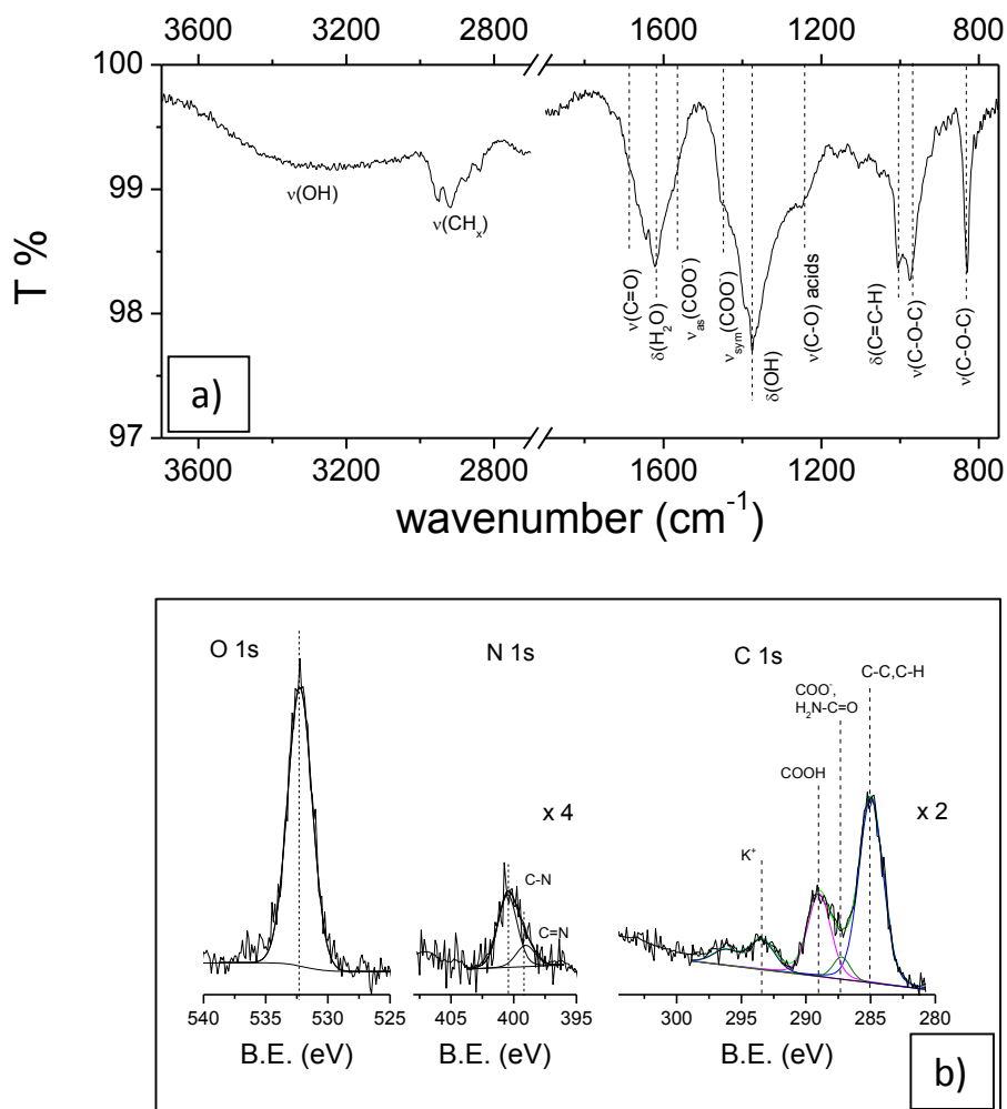
Fig. 2. a) FT-IR and b) XPS analyses.
