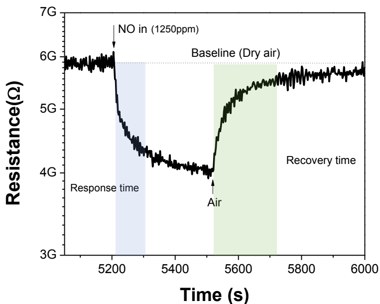
Fig. 6. Transient response of the C-CDs sensor.
