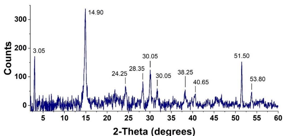
Fig. 1. XRD pattern of C-CDs
