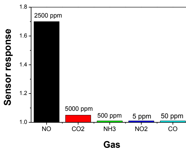
Fig. 9. Response of the C-CDs based sensor to different gases. The high response to NO, compared with the lower response to other gases, highlights the high selectivity of this sensor towards NO.
