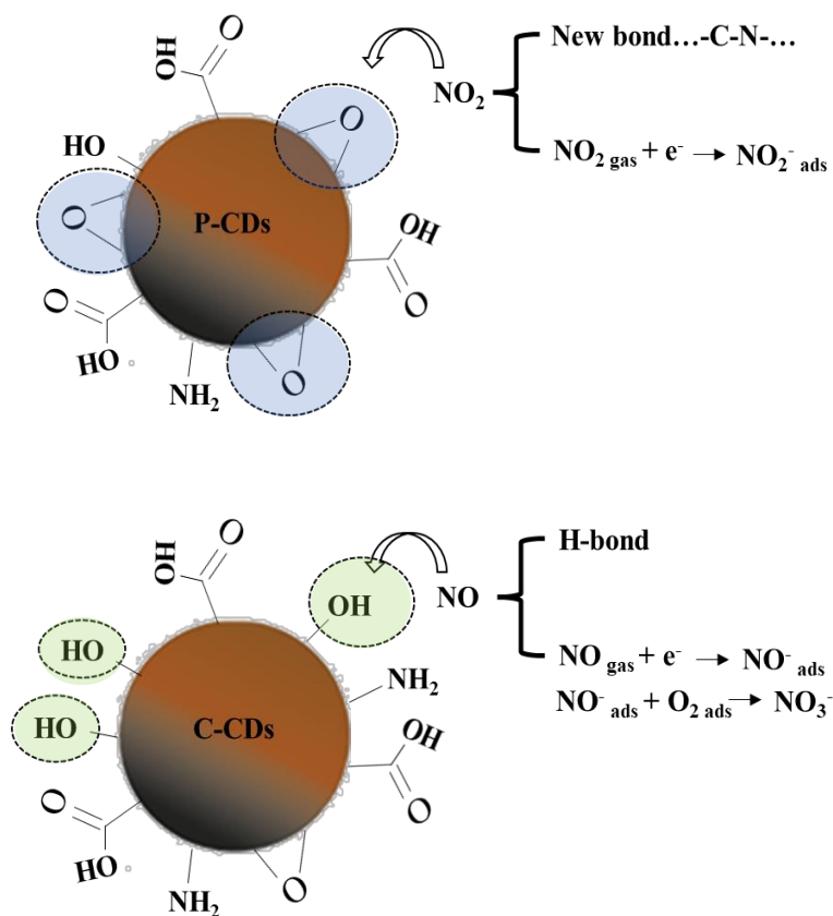
Fig. 11. Schematic representation of the NO and NO 2 sensing mechanism on C-dots sensors.
