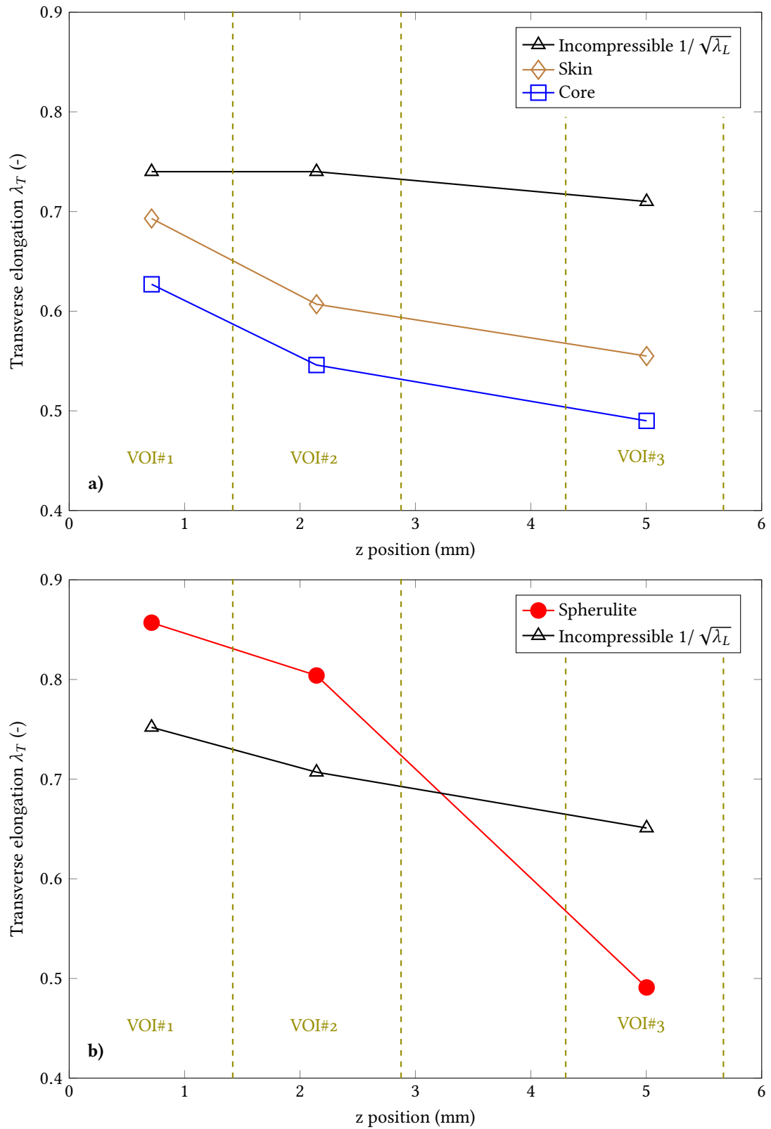
Figure 13: Evolution of the transverse elongations ( \lambda_T ) along the necked region: a) Core and skin; b) at the spherulitic scale
