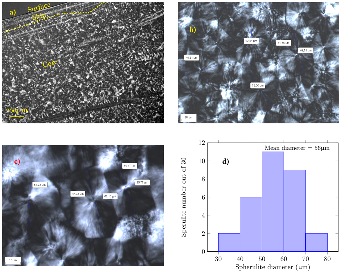
Figure 2: Optical microscopy examination of the spherulites on microtomed thin film of the PP under study: a) Large surface; b) and c) Focuses on smaller surfaces to allow diameter measurements; d) Histogram of the spherulite diameter measured on 30 net spherulites
