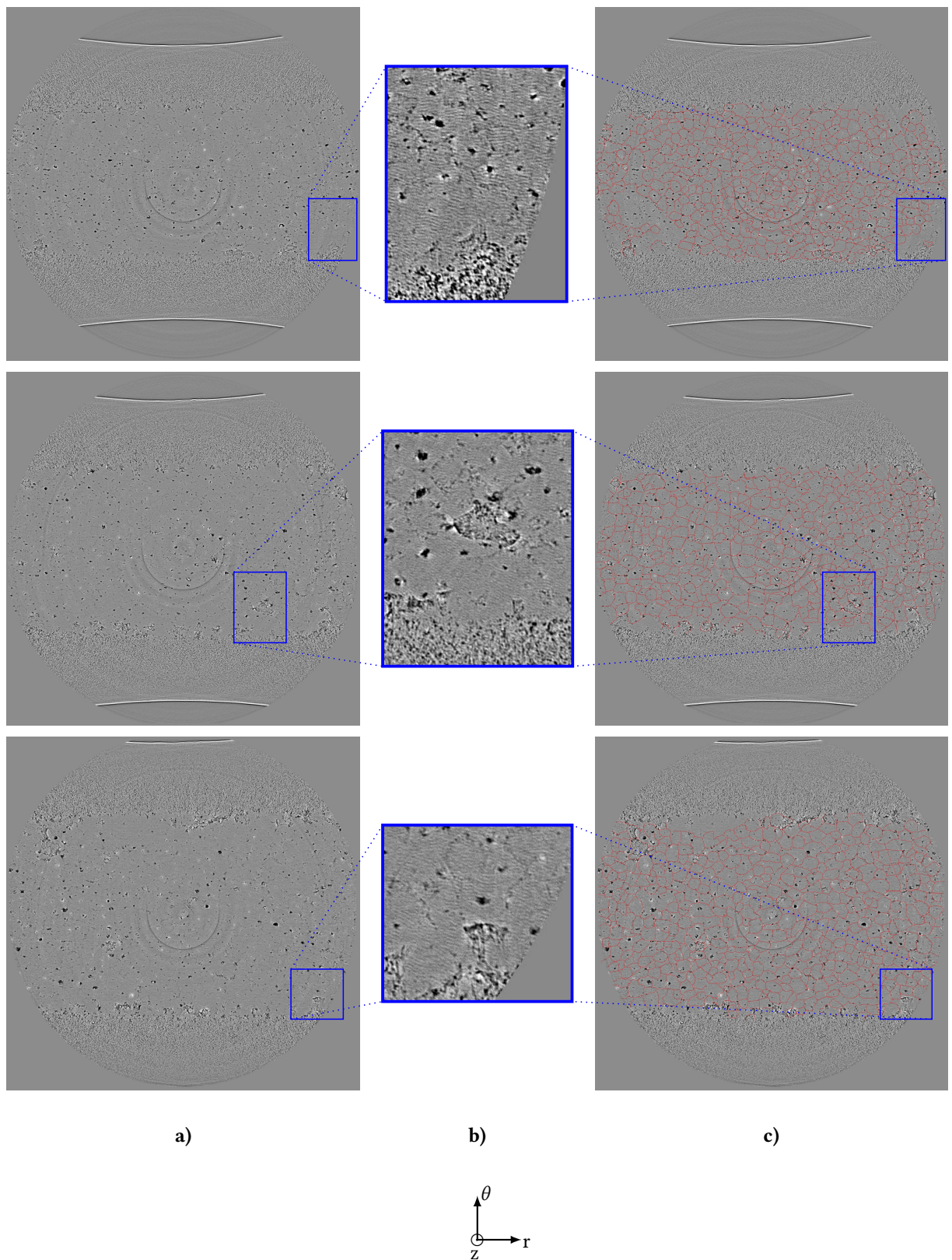
Figure 8: 2D section top views of microtomography data of the three VOIs' presented in fig. 3 so as to determine the diameters of the deformed spherulites: a) Reconstructed images; b) Closer examinations of a specific region; c) Drawings of the identified boundaries for the deformed spherulites
