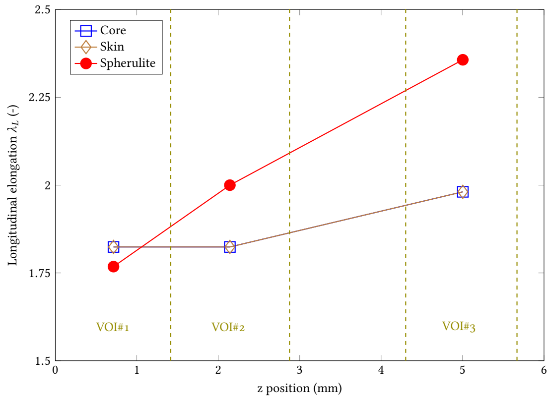
Figure 12: Evolution of the longitudinal elongations ( \lambda_L ) along the necked region
