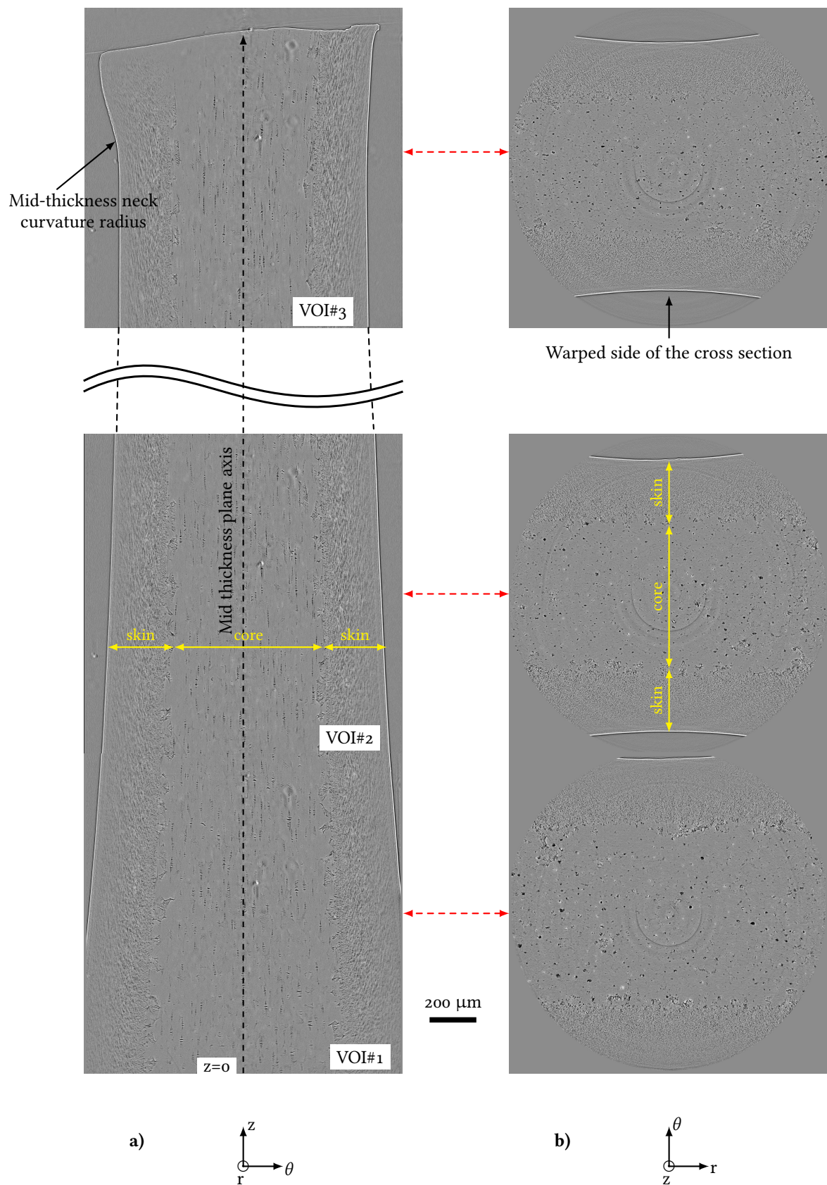
Figure 3: The three microtomography data sets representative of the Volumes of interest (VOI): a) Side views at mid-width cuts; b) Corresponding top views of respective VOIs'. Yellow arrows indicate the core/skin regions allowing their thicknesses to be measured
