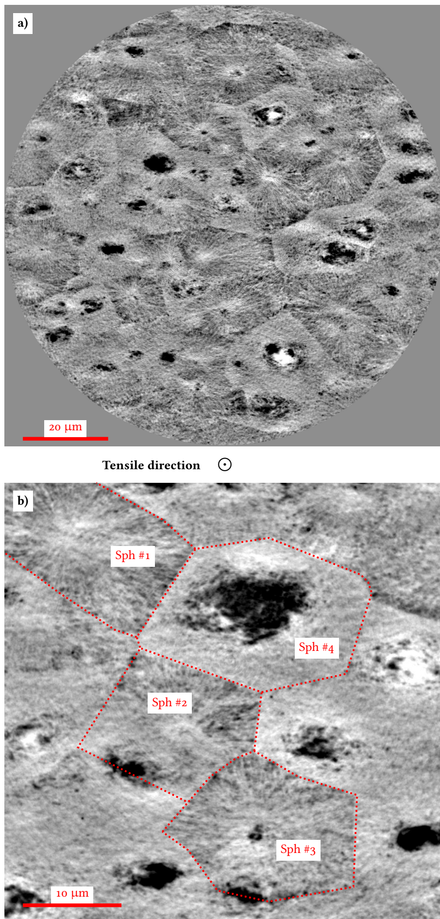
Figure 7: Top views of data set of deformed PP at a resolution of 50 nm: a) global view 102 \mu\text{m} x 102 \mu\text{m} ; b) closer look at few spherulites: 45 \mu\text{m} x 45 \mu\text{m}
