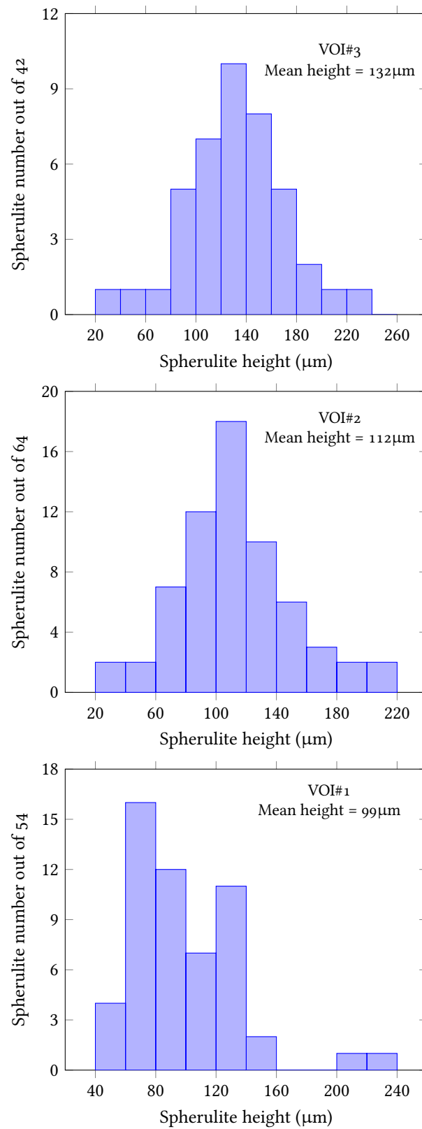
Figure 11: Histograms of the heights of the identified polar fans in the core along the z-direction, for VOIs' #1,2,3 from bottom to top.
