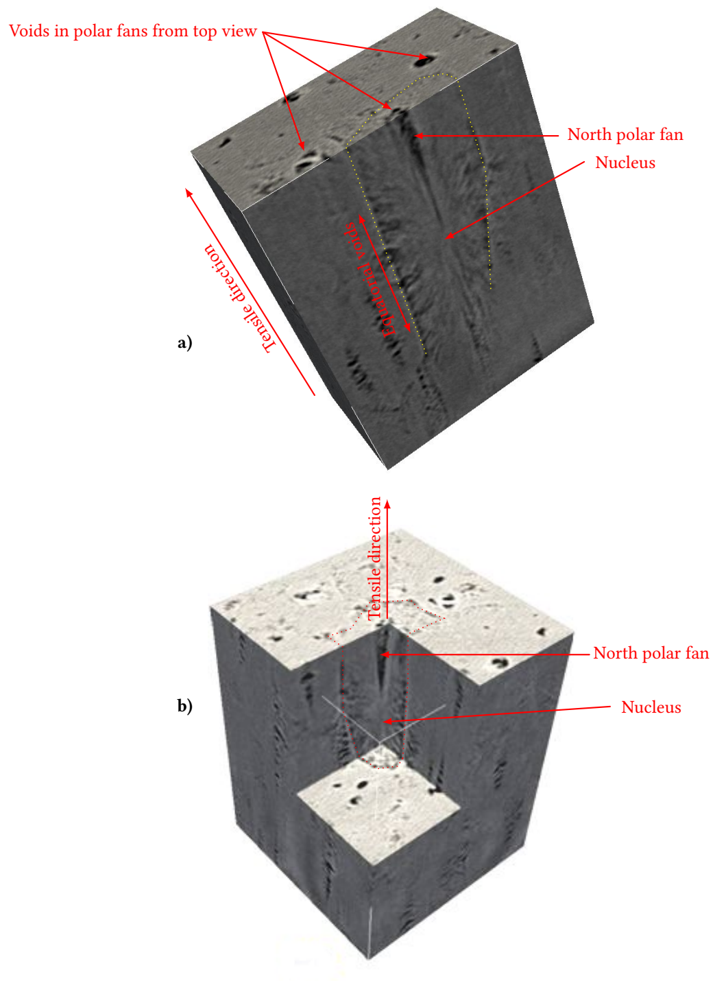
Figure 5: Various 3D views of deformed spherulites showing polar fans, from data sets obtained from Synchrotron Radiation Tomography with a resolution corresponding to 1 pixel size \approx 0.7\mu\text{m} . Cube side about 140\mu\text{m}
