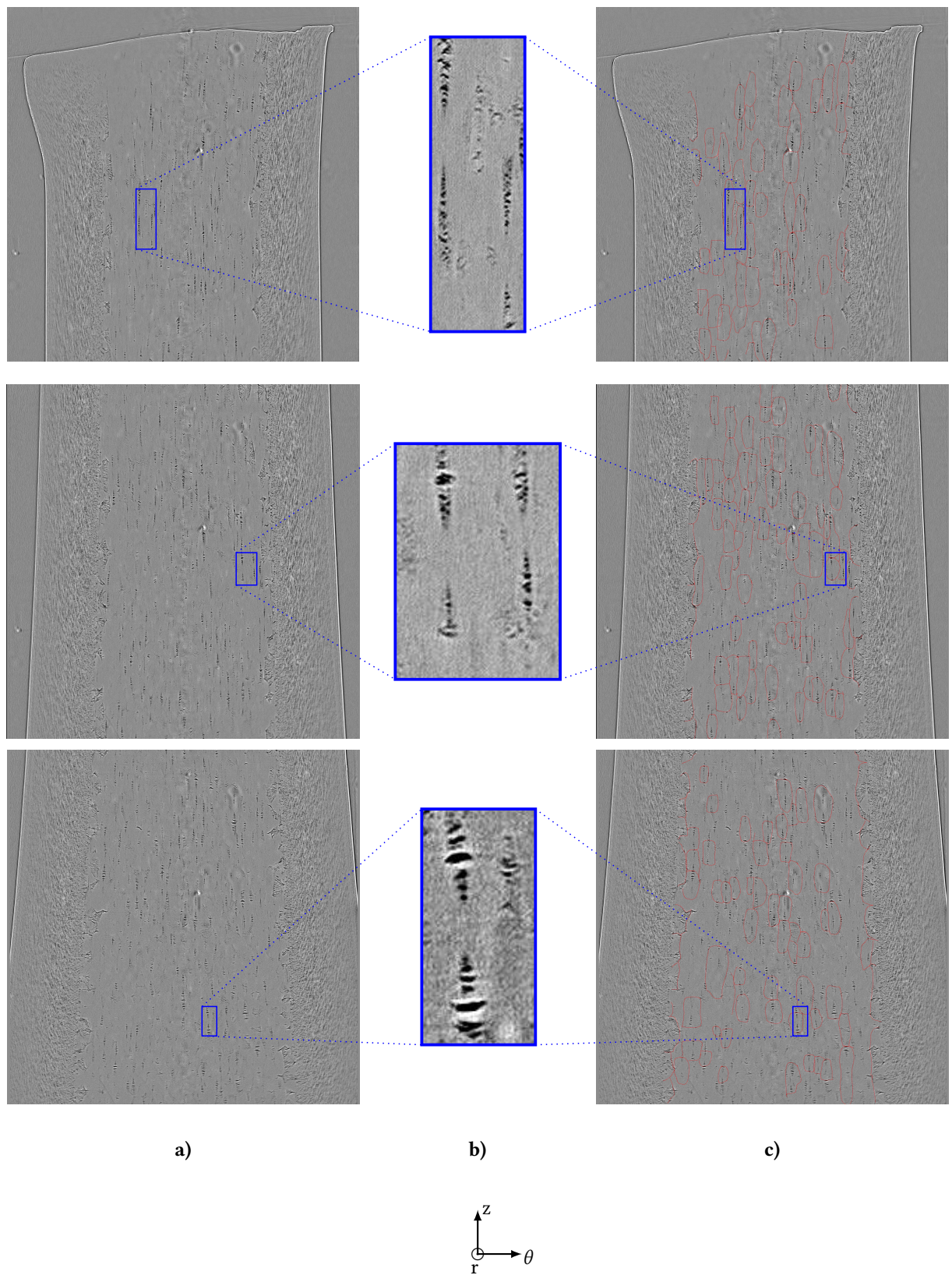
Figure 9: Side views of the three VOIs' presented in fig. 3 so as to determine the heights of the deformed spherulites: a) Reconstructed images; b) Closer examinations of a specific region; c) Drawings of the identified polar fans inside the deformed spherulites
