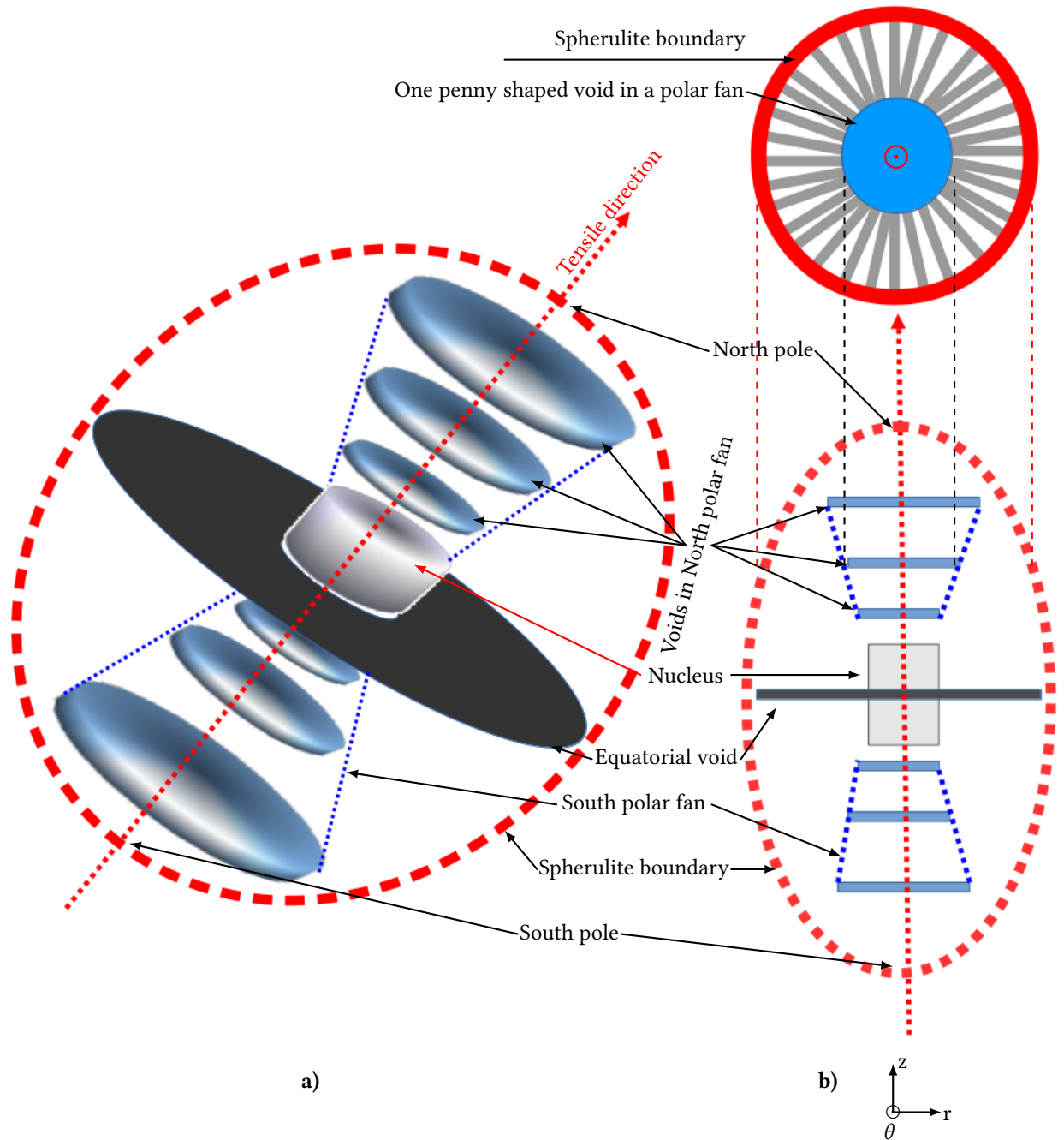
Figure 1: Idealized views of a deformed spherulite: a) Perspective view in 3D; b) 2D views from longitudinal cut (side view) and cross section cut (top view). Cylindrical coordinates related to the side view is shown below fig.1.b)
