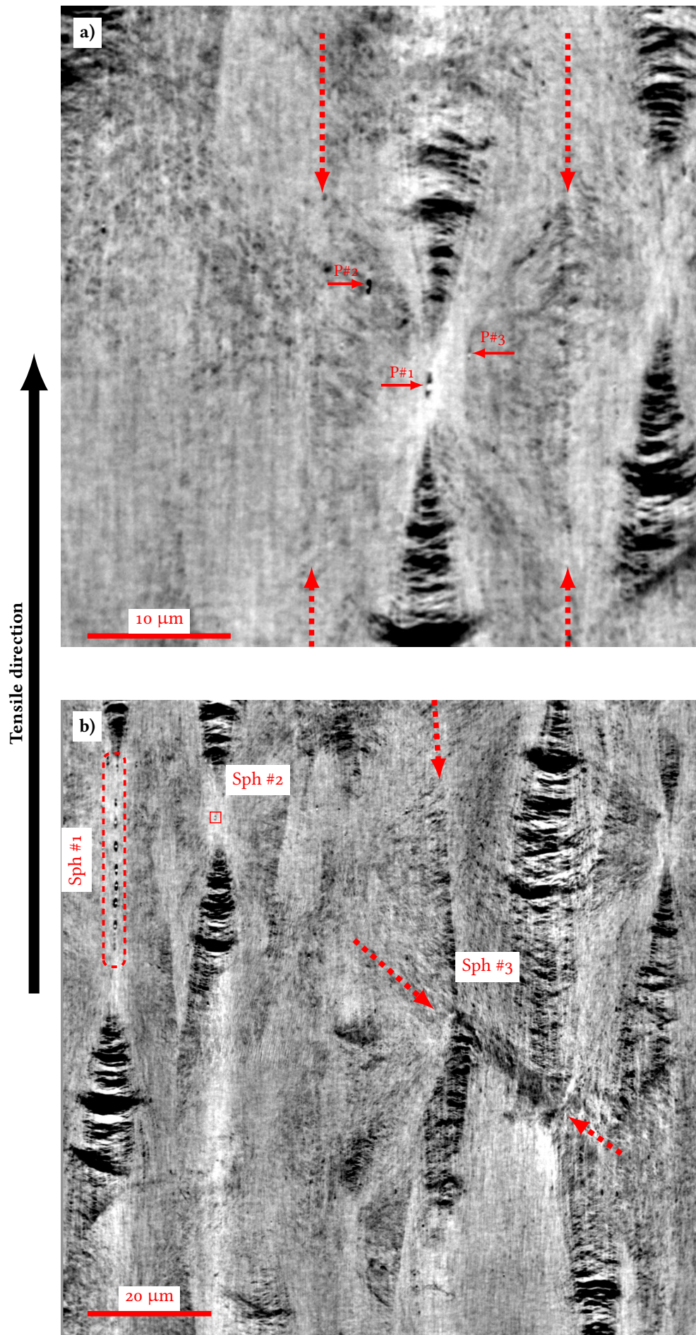
Figure 6: Side views of the data set of deformed PP at a resolution of 50 nm: a) detailed view of a couple of polar fans; b) global view 102 μm x 102 μm.
