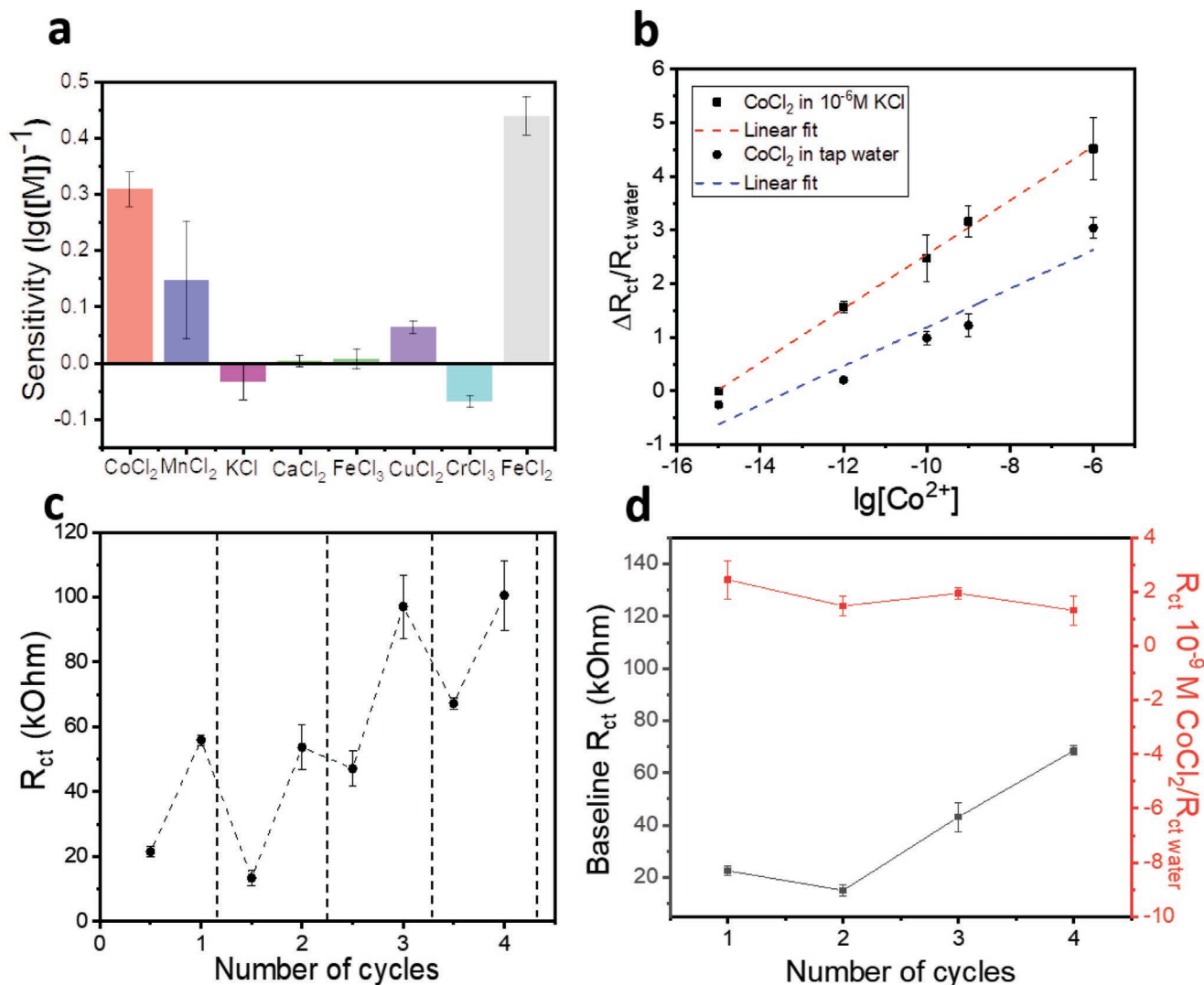
Figure 3. a) Comparison of device sensitivity to the change of concentration for Co 2+ and interfering cations. [M] is the concentration of a given cation. b) Normalized charge transfer resistance response as a function of CoCl 2 concentration with the fixed 10 -6 M KCl concentration (red) and in tap water (blue). The normalization was performed by the device's R ct in MQ water. c) R ct change as a function of sensing/washing cycles. d) Normalized charge transfer resistance for the detection of Co 2+ (red) and baseline variation (black) as a function of number of cycles.
