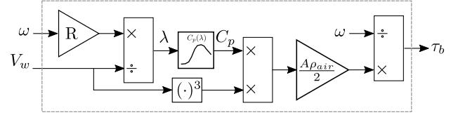
Fig. 8. Aerodynamics simulator scheme.
