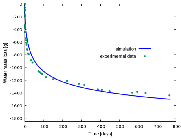
Fig. 4. Water mass loss of the cylindrical concrete sample. Experimental data and simulated curve issued from the FEM computation.
