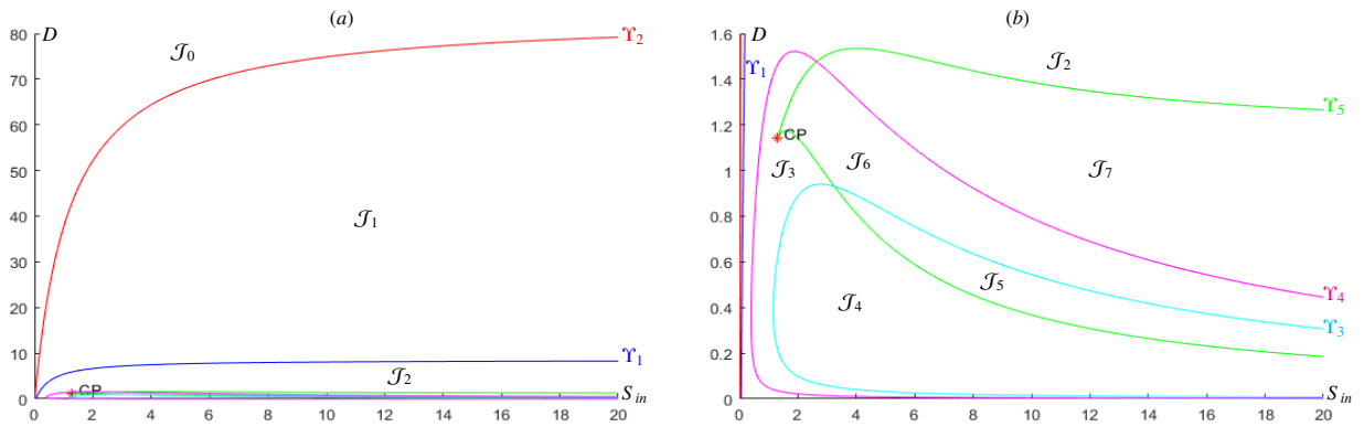
Figure 5: MATCONT: (a) operating diagram of (2). (b) Magnification showing the cusp bifurcation when (S_{in}, D) \in [0, 20] \times [0, 1.6] .
