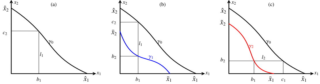
Figure 1: (a-b-c) Definitions of the functions x_2 = G(x_1) , x_2 = F_1(x_1) and x_1 = F_2(x_2) , and the corresponding graphs \gamma_0 , \gamma_1 and \gamma_2 (in black, blue and red), respectively.
