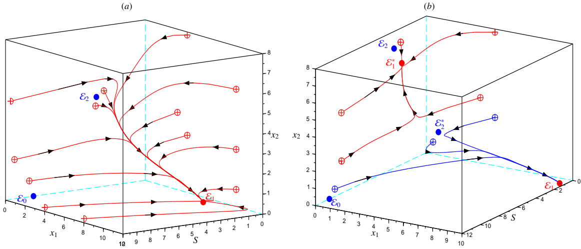
Figure 11: SCILAB: the three-dimensional space (S, x_1, x_2) of (27) when D = 5 : (a) S_{in} = 8 < S_{in}^c \approx 9.357 , convergence to \mathcal{E}_1 . (b) S_{in} = 10.5 > S_{in}^c , bistability with either convergence to \mathcal{E}_1 or \mathcal{E}_1^* .
