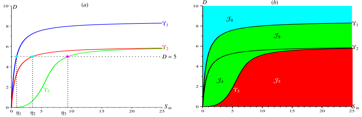
Figure 8: MAPLE: (a) the three curves \Upsilon_1 , \Upsilon_2 and \Upsilon_5 in the (S_{in}, D) -plane. (b) The corresponding operating diagram of model (27).
