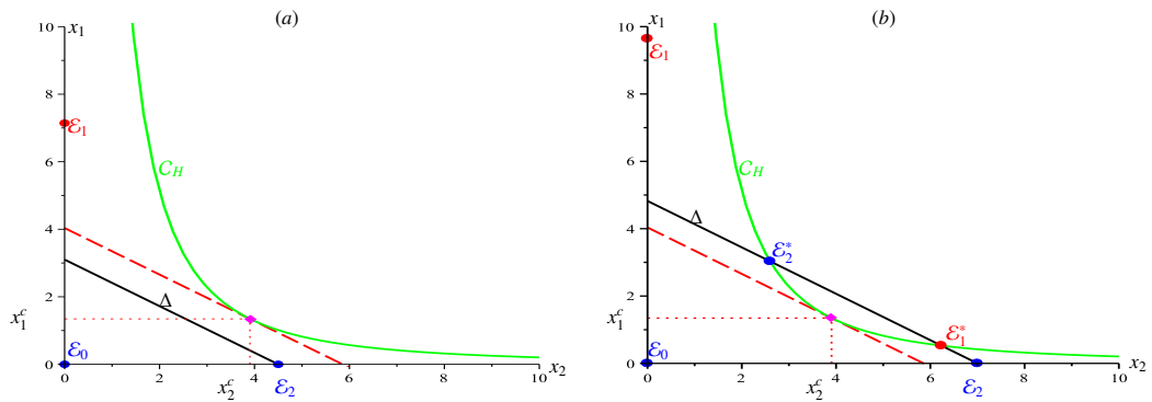
Figure 7: Existence and stability of steady states of model (27) when D = 5 : (a) S_{in} = 8 < S_{in}^c \approx 9.357 , (b) S_{in} = 10.5 > S_{in}^c . In all figures, we use the red [resp. blue] color for LES [resp. unstable] steady state.
