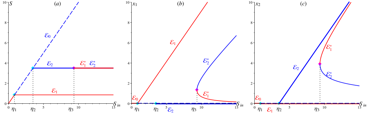
Figure 9: MAPLE: (a-b-c) one-parameter bifurcation diagrams of system (27) in the variables S , x_1 , x_2 , (resp.), with S_{in} as the bifurcation parameter and D = 5 .
