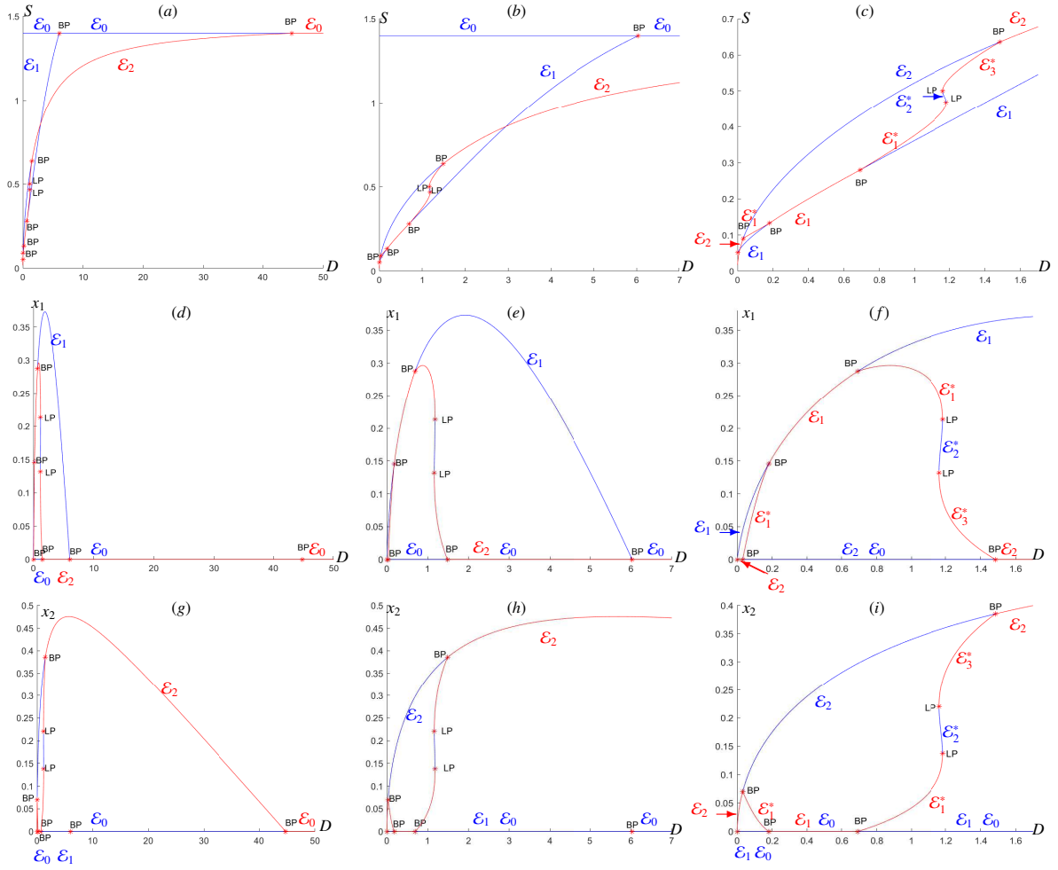
Figure 6: MATCONT: (a-d-g) one-parameter bifurcation diagrams of (2) in the variables S , x_1 , x_2 , (resp.), with D as the bifurcation parameter and S_{in} = 1.4 ; (b-e-h) (resp. (c-f-i)) magnifications when D \in [0, 7] (resp. D \in [0, 1.7] ); Red (resp. Blue) curve represents the continuation of a stable (resp. unstable) steady state.
