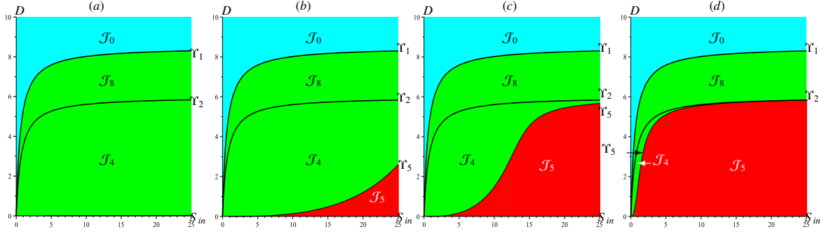
Figure 10: MAPLE: effect of the variation of the parameter \alpha_1 on the emergence of the coexistence region with bistability in the operating diagram of (27): (a) \alpha_1 = 10^{-5} , (b) \alpha_1 = 10^{-3} (c) \alpha_1 = 10^{-2} , (d) \alpha_1 = 20 .
