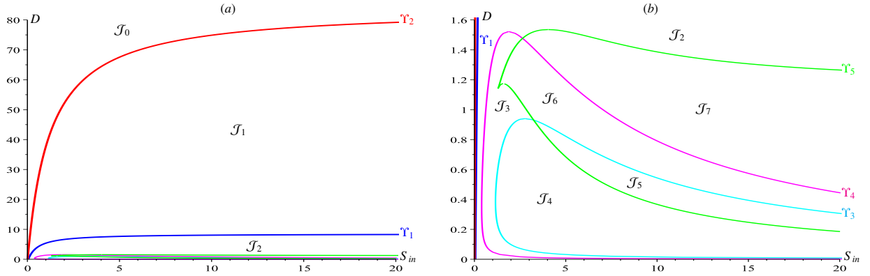
Figure 4: MAPLE: (a) operating diagram of (2). (b) Magnification when (S_{in}, D) \in [0, 20] \times [0, 1.6] .
