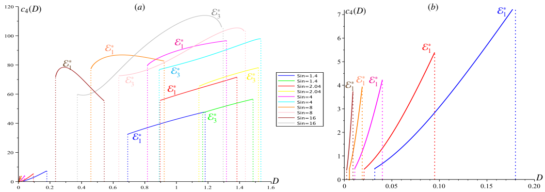
Figure B.12: MAPLE: (a) curves of the function c_4(D) corresponding to \mathcal{E}_1^* [resp. \mathcal{E}_3^* ] for all D in their existence domain (\sigma_3, \sigma_5) [resp. (\sigma_4, \sigma_6) ] when S_{in} = 1.4 and S_{in} = 2.04 , and in (\sigma_4, \sigma_3) [resp. (\sigma_6, \sigma_5) ] when S_{in} = 4 , S_{in} = 8 , and S_{in} = 16 . (b) Magnification of c_4(D) corresponding to \mathcal{E}_1^* for all D \in (\sigma_1, \sigma_2) .
