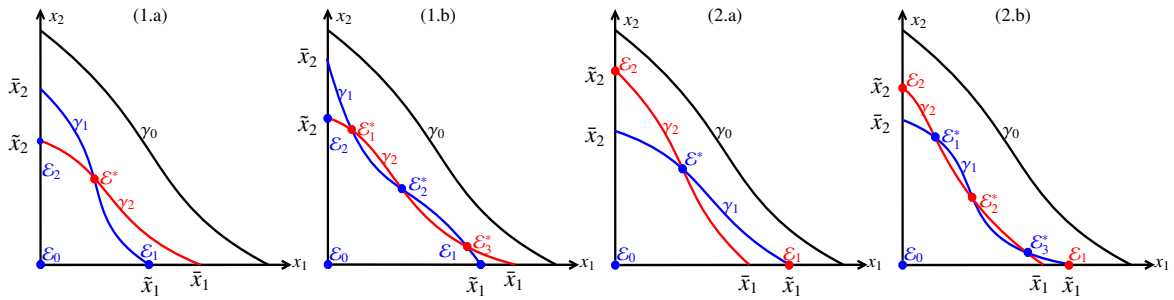
Figure 2: Case 1 : \bar{x}_1 > \bar{x}_1 and \bar{x}_2 > \bar{x}_2 ; Case 2 : \bar{x}_1 < \bar{x}_1 and \bar{x}_2 < \bar{x}_2 : (a) unique intersection, (b) an odd number of intersections.
