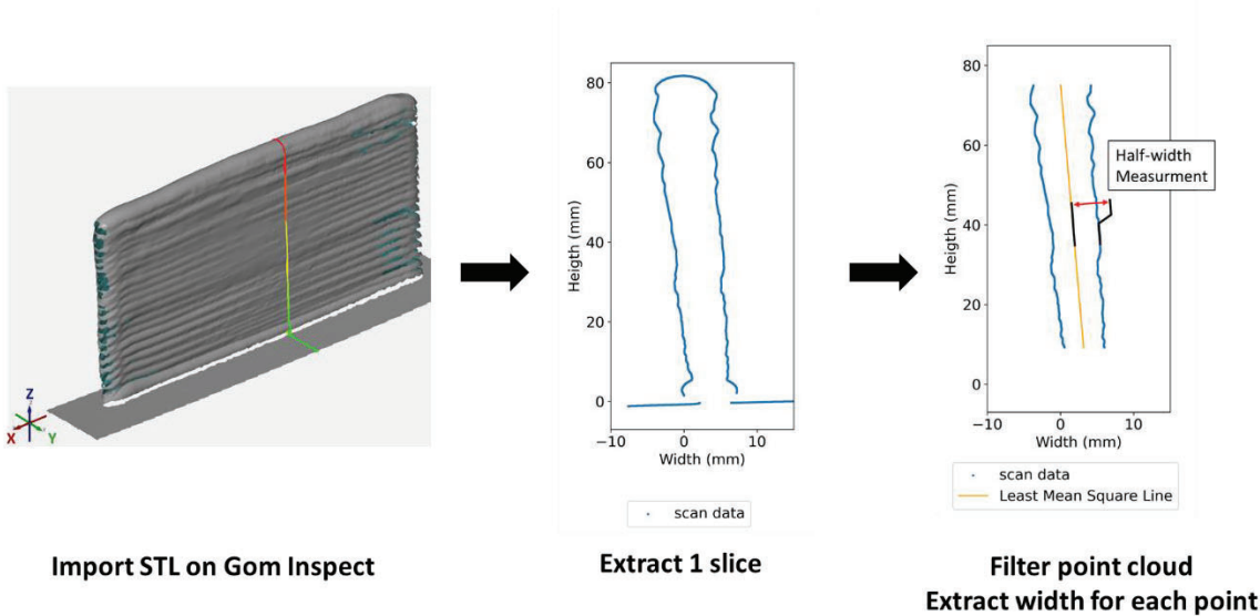
Figure 11: Width extraction method
