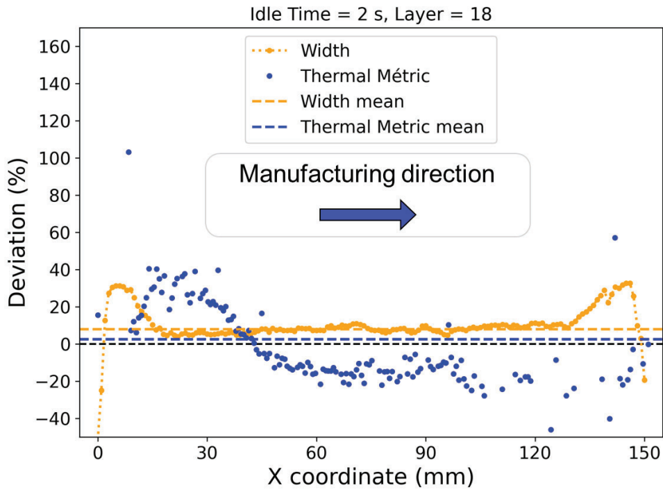
26 a) Layer 18, Idle time = 2s. Referent width is 5.81 mm
