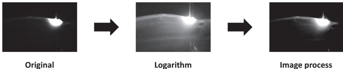
Figure 7: Image Process
