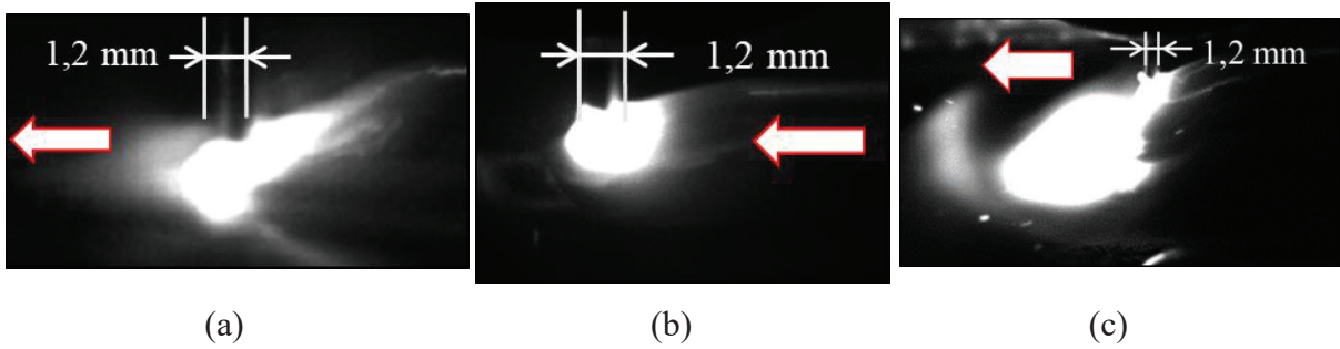
Figure 5: Example of images function of the delay and the exposure time. (a) Shorten delay, (b) a correct image, (c) an image with too much delay or exposure time.
