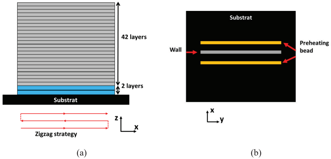
Figure 2: Manufacturing strategy (a) Side view, (b) Top view
