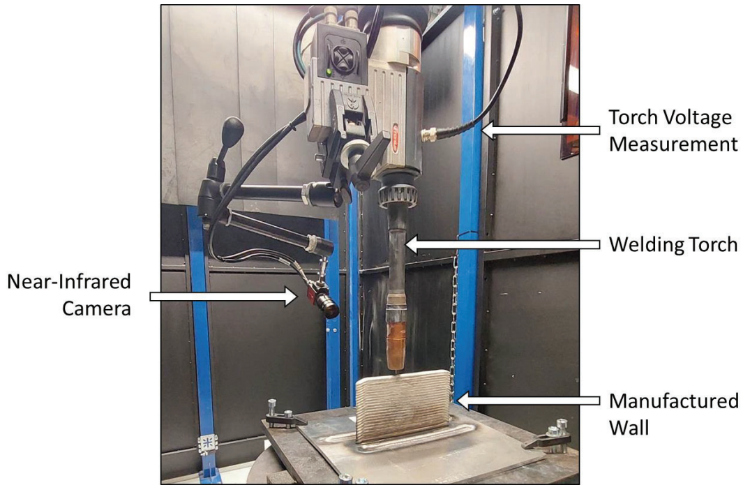
Figure 3: camera fixation on the torch
