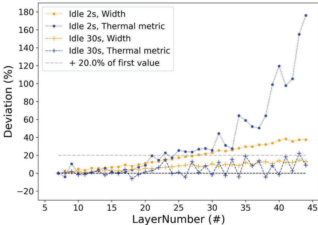
Figure 12: Mean width deviation and mean normalized thermal metric as a function of the layer number for the two wall. For the 2 seconds idle time wall, the reference width is equal to 5.81 mm. For the 30 seconds idle time wall, the reference width is equal to 5.33 mm.
