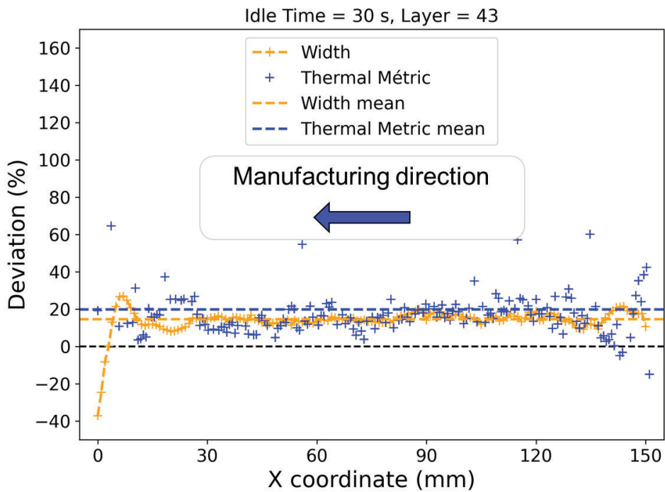
53 b) Layer 43, Idle time = 30s, Referent width is 5.33 mm
