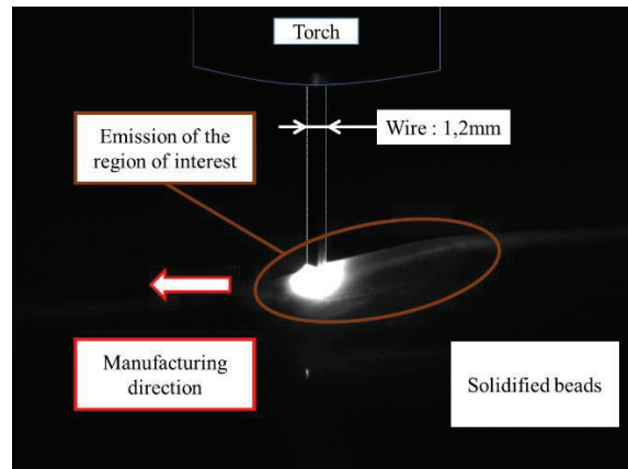
Figure 4: Typical image obtained with the NIR camera
