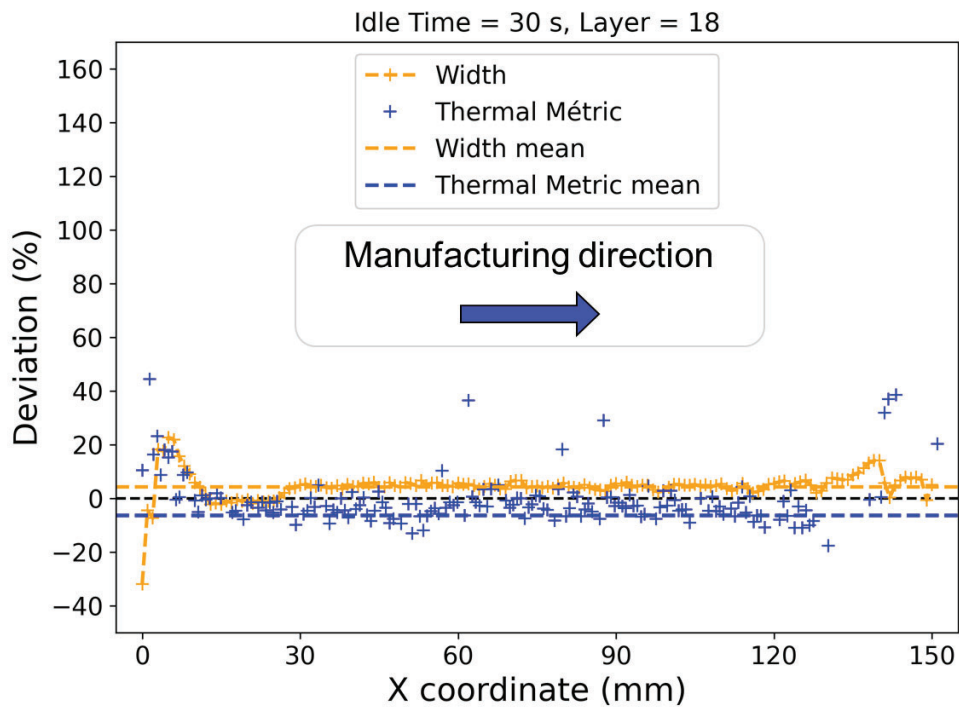
26 a) Layer 18, Idle time = 30s, Referent width is 5.33 mm
