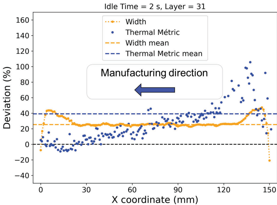
53 b) Layer 31, Idle time = 2s, Referent width is 5.81 mm
