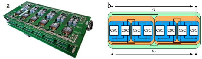
2.5. Fig. 5. Product architecture of the PCA (a) and its topology (b) [28]. Link Between Modular Design and Modularity in PEC
